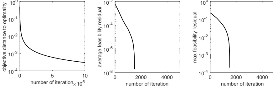
FIG. 1. Results given by Algorithm 1 with nonadaptive setting on solving an instance of the sample approximation (5.2) of the robust portfolio selection. Left: the distance of objective value at averaged point to optimal value |f_0(\bar{\mathbf{x}}^k) - f_0(\mathbf{x}^*)| ; Middle: the average constraint violation at averaged point \frac{1}{M} \sum_{j=1}^M [f_j(\bar{\mathbf{x}}^k)]_+ ; Right: the maximum constraint violation at averaged point \max_{j \in [M]} [f_j(\bar{\mathbf{x}}^k)]_+ .
