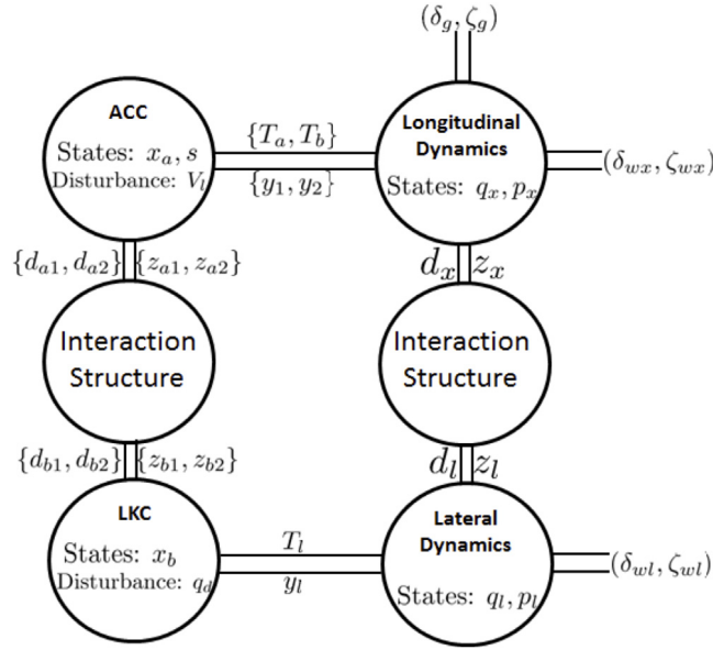
Fig. 4. Closed-loop system.
