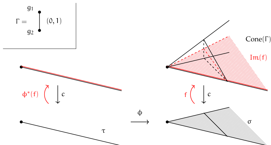
Figure 9. The tropical curve \Gamma over \sigma , on the northwest corner of the figure, consists of one edge of length (0, 1) and two vertices of genera g_1 and g_2 . The right hand side of the picture depicts \text{Cone}(\Gamma) , with the structure morphism c and the section f(x, y) = (x, y, y/2) . The face morphism \phi : \tau \rightarrow \sigma is illustrated on the left hand side. The tropical curve \Gamma_\tau consists of a vertex of genus g_1 + g_2 , and therefore \text{Cone}(\Gamma_\tau) is itself a ray. Observe that H(f) = 0 , while H(\phi^*(f)) = g_1 + g_2 .
