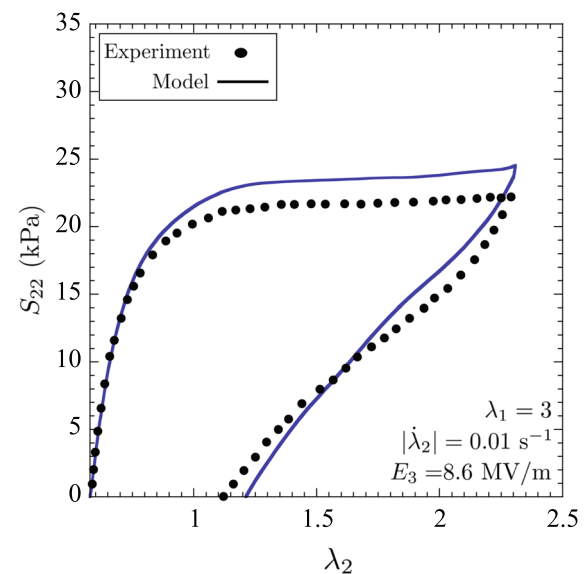
Fig. 4 Load/unload response of uniaxially pre-stretched ( \lambda_1 = 3 ) VHB 4910 subject simultaneously to a uniaxial stretch \lambda_2 perpendicular to the pre-stretch direction, applied at the constant stretch rate of |\dot{\lambda}_2| = 0.01 s ^{-1} , and a constant Lagrangian electric field E_3 = 8.6 MV/m. The solid circles correspond to the experimental data of Hossain et al. [20], while the solid line corresponds to the response predicted by the model with the material parameters listed in Table 1
