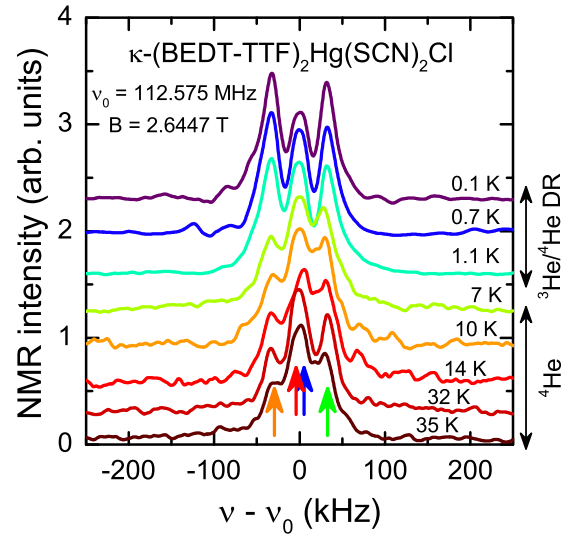
FIG. 2. The shape and width of the ^1\text{H} NMR spectra remain unaffected upon cooling through T_{CO} = 30 \text{ K} , ruling out magnetic order down to millikelvin temperatures. The NMR intensity was normalized with respect to the 1/T enhancement; curves were shifted vertically. The minor difference in line shape below and above 2 K is due to slightly different sample alignment in the ^3\text{He}/^4\text{He} dilution refrigerator ( T < 2 \text{ K} ) and the ^4\text{He} flow cryostat (2–100 K) [44].
