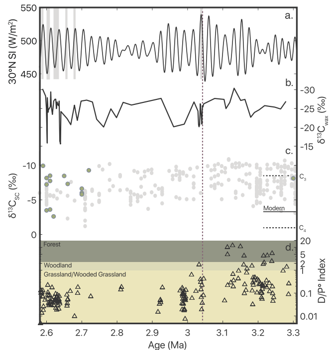
Fig. 5. BTB13 \delta^{13}\text{C}_{\text{wax}} (b) compared to mean summer 30°N insolation (a; Laskar et al., 2004 ) containing the characteristic diatomaceous sequence from the Chemeron Formation (light grey bands) in the Baringo Basin ( Deino et al., 2006 ; Kingston et al., 2007 ). Wax isotopes are further contextualized with \delta^{13}\text{C}_{\text{SC}} measurements (c) from the Baringo Basin (green circles; Kingston et al., 1994 ; Kingston, 1999 ) and the East African compilation (grey circles; Levin, 2013 and references therein). C 3 and C 4 endmembers (dashed lines) and modern value from the Baringo Basin demonstrate that the late Pliocene was on average more C 3 -dominated than today (c). Vegetation reconstructions from the ratio of tree:grass phytoliths (triangles; Yost et al., this issue ) produce an index of tree cover D/P° (d). The D/P° index ( Bremond et al., 2008 ) is a proxy for tree canopy cover in Africa and has been applied to determine vegetation structure, with vegetation formation classifications after White (1983) . The changepoint-derived shift in vegetation at ~3.04 Ma is denoted in purple dashed line. (For interpretation of the references to colour in this figure legend, the reader is referred to the Web version of this article.)
