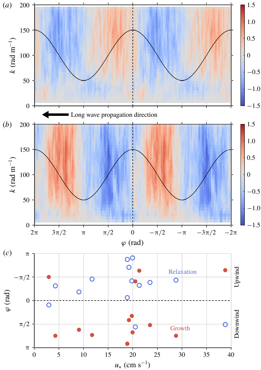
FIGURE 14. Variation of downwind short wave growth rate \beta(k, \varphi) in units of s^{-1} : (a) low energy wave field, low wind forcing of u_* = 19.8 cm s^{-1} , (b) well-developed wind sea, moderate wind forcing of u_* = 38.8 cm s^{-1} . Example long wave shapes are overlaid as black curves for reference, with the vertical dashed lines marking the position of the wave crest. The downwind/long wave propagation direction is indicated by the black arrow. (c) Variation in the long wave phase of peak short wave growth/relaxation with respect to air-side friction velocity. Filled red circles indicate wave growth; open blue circles indicate wave relaxation.
