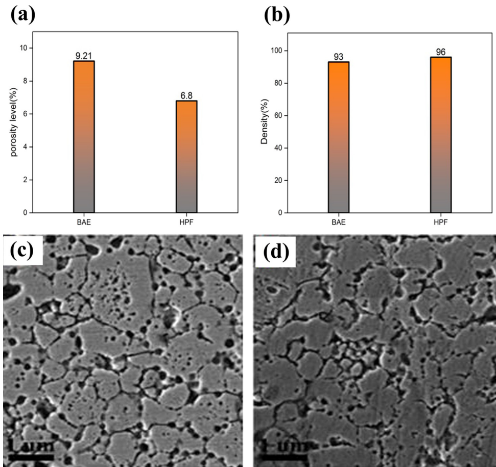
Fig. 6. A) Percentage of the porosity, obtained from image analysis BAE and HPF sample. B) Percentage of density BAE and HPF sample. C) FE-SEM images of the specimens after etching for BAE sample. D) FE-SEM images of the specimens after etching for HPF sample.
