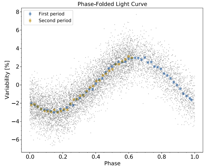
Figure 5. The Spitzer light curve of VHS1256b folded to the best-fitting period of 22.04 hr. The blue and yellow squares are binned photometric points in the first and second period, respectively. The light curves spanning the two periods are in excellent agreement with each other.
