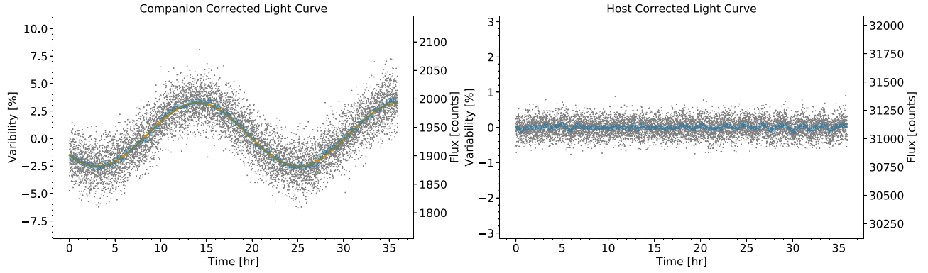
Figure 4. Light curves of VHS1256b and VHS1256AB after pixel-mapping corrections. Systematic trends presented in Figure 3 are eliminated for the companion and the host. Although we assume single sine wave models for both objects at the beginning of the iterative correction, their final corrected light curves are different. The corrected light curve of the companion has a sinusoidal modulation with an amplitude of 5.76%. The corrected light curve of the host agrees with a flat line except for a low-level ( <0.1\% ) periodic variation in the third AOR.
