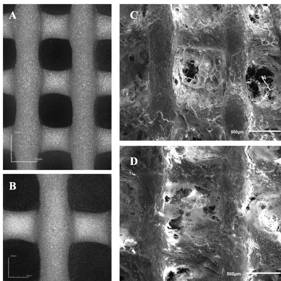
Fig. 4 – 3D laser scanning micrographs of the 3D-printed \beta -TCP scaffold (A, B), Scanning electron micrographs of (C), Col-Hep and (D), Col-Hep-rhBMP2 matrices encapsulating MSCs filled into the 3D printed \beta -TCP scaffolds after 21 days (A, B: scale bar is 500 \mu m).
