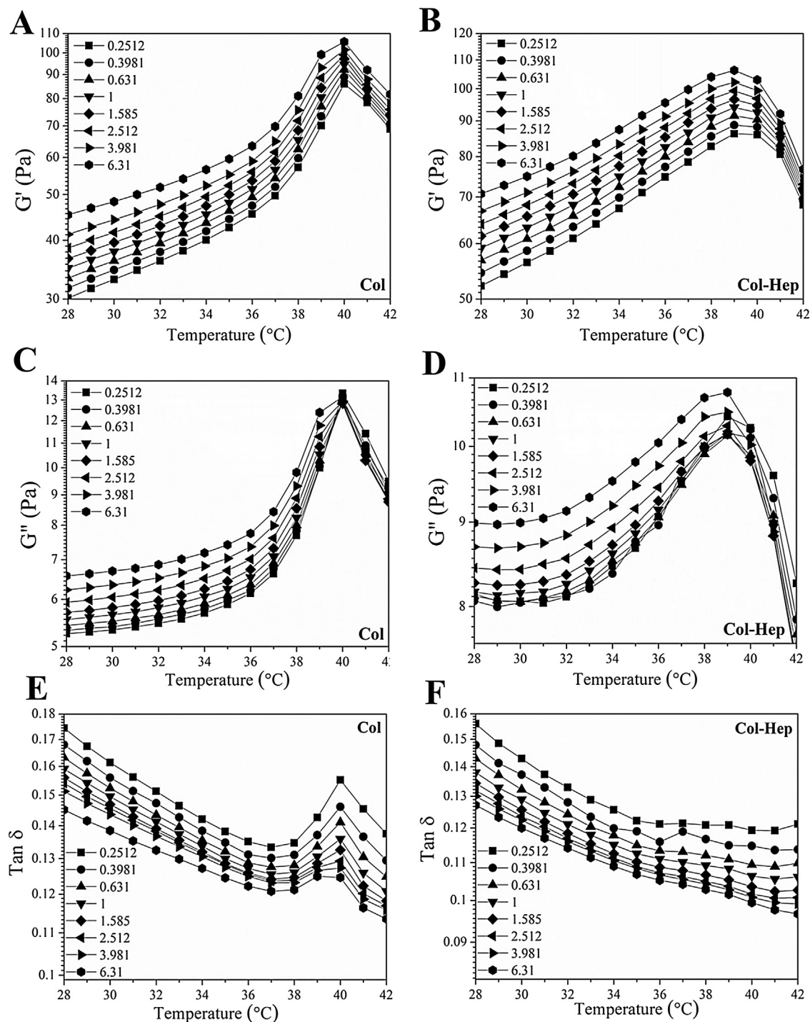
Fig. 2 – Rheological characterization of Col and Col-Hep matrices: storage modulus ( G' ) as a function of temperature at the indicated frequencies for (A) Col, and (B) Col-Hep matrices. Thermal evolution of the loss modulus ( G'' ) for (C) Col, and (D) Col-Hep matrices. Temperature-induced evolution of the viscoelastic loss tangent ( \tan\delta ) for (E) Col, and (F) Col-Hep matrices.
