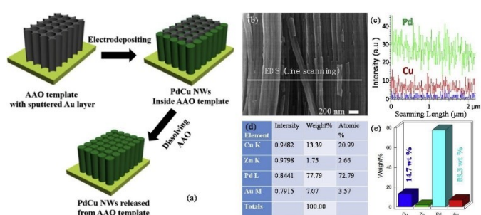
Fig. 3. (a) Schematic of Pd/Cu NW array fabrication, (b) SEM image of Pd/Cu NW arrays. The inset line indicates the position where the EDS line scan was taken. (c) The corresponding elemental mapping from (b). (d–e) The summarized elemental analysis of Pd/Cu NWs, obtained from the EDS line scan in (b). Zn and Au are from the substrate holder and the Au layer sputtered onto the AAO template, respectively. Reproduced with permission. 37 Copyright 2019 Springer
