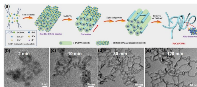
Fig. 13 Formation mechanism of ultrathin PdCuP nanowires. (a) Schematic illustration of growth mechanism of ternary PdCuP NWs using DODAC as the surfactant template and NaH 2 PO 2 as reducing agent and P source. Representative PdCuP alloy TEM images obtained at reaction times of (b) 2 min, (c) 10 min, (d) 30 min, and (e) 120 min. Reproduced with permission. 88 Copyright 2019 Elsevier
