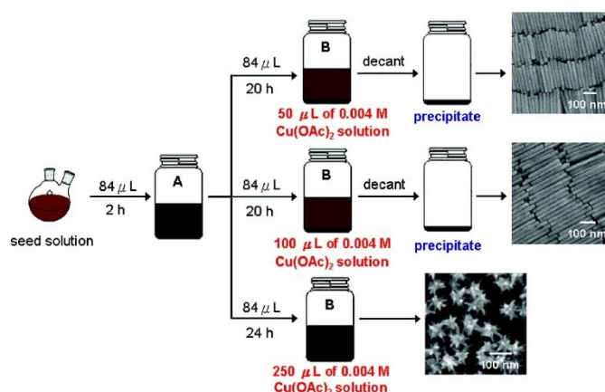
Fig. 7 Experimental procedure used to make palladium nanorods and branched nanocrystals. Reproduced with permission. 53 Copyright 2009 American Chemical Society
