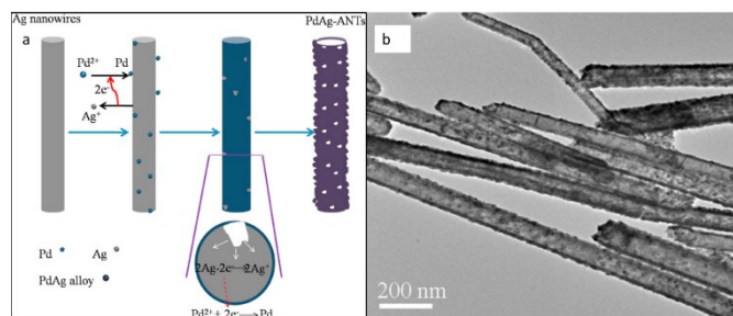
Fig. 9 (a) Schematic illustration showing the synthesis process of PdAg alloy nanotubes via galvanic replacement of Ag nanowires. (b) TEM image of PdAg alloy nanotubes. Reproduced with permission. 160 Copyright 2017 Elsevier.
