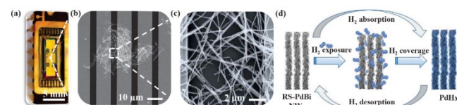
Fig. 21 (a) Hydrogen sensor prototype. (b, c) Sequentially magnified SEM images of the interdigitated electrode integrated with multiple rough-surface (RS)-PdBi NWs. (d) Schematic illustration of the RS-PdBi NWs for H 2 adsorption and desorption cycles. Reproduced with permission. 21 Copyright 2019 American Chemical Society.
