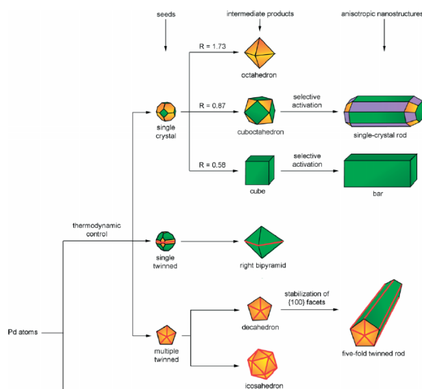
Fig. 11 A schematic illustration different morphologies of Pd nanostructures and conditions leading to them. Reproduced with permission. 12 Copyright from Wiley-VCH.
