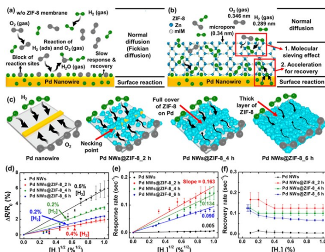
Fig. 20 Schematic illustration of Pd NWs@ZIF-8 hydrogen sensor. a) Sensing model for Pd NWs without ZIF-8 membrane, and b) sensing model for Pd NWs@ZIF-8. Without ZIF-8, H 2 sensing can be significantly affected by oxygen in air. In the presence of ZIF-8, O 2 diffusion is limited. (c) Fabrication of Pd@ZIF-8 at different time interval; Pd NW, Pd NWs@ZIF-8_2 h, Pd NWs@ZIF-8_4 h, and Pd NWs@ZIF-8_6 h. (d) Response vs [H 2 ] 0.5 in air, (e) response rate vs [H 2 ] 0.5 in air, and (f) recovery rate versus [H 2 ]. Reproduced with permission. 25 Copyright 2017 American Chemical Society.
