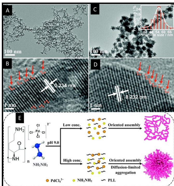
Fig. 14. (A) and (B) TEM and HRTEM images of Pd nanowires; (C) and (D) TEM and HRTEM images of dendrite-like Pd nanoparticles obtained at higher PLL conc. (E) The proposed formation mechanism of Pd NCNs and Pd NDs via surfactant based self-assembly. Reproduced with permission. 89 Copyright 2018 Elsevier.
