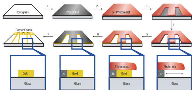
Fig. 2 Seven-step process flow for metal-nanowire fabrication using LPNE. Reproduced with permission. 171 Copyright 2006 Springer Nature.
