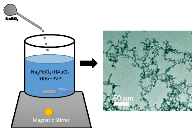
Fig. 10 Schematic of PdAu nanowire networks synthesis using chemical reduction method; (b) TEM images of PdAu nanowire network. Adapted with permission. 82 Copyright 2014 American Chemical Society
