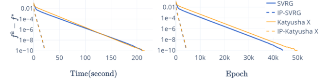
Figure 5.9. Sum-of-nonconvex on synthetic data. \lambda_1 = 10^{-3} , \alpha = 15, \eta_1 = 0.015, \eta_2 = 10^{-4}, \tau = 0.45 .
