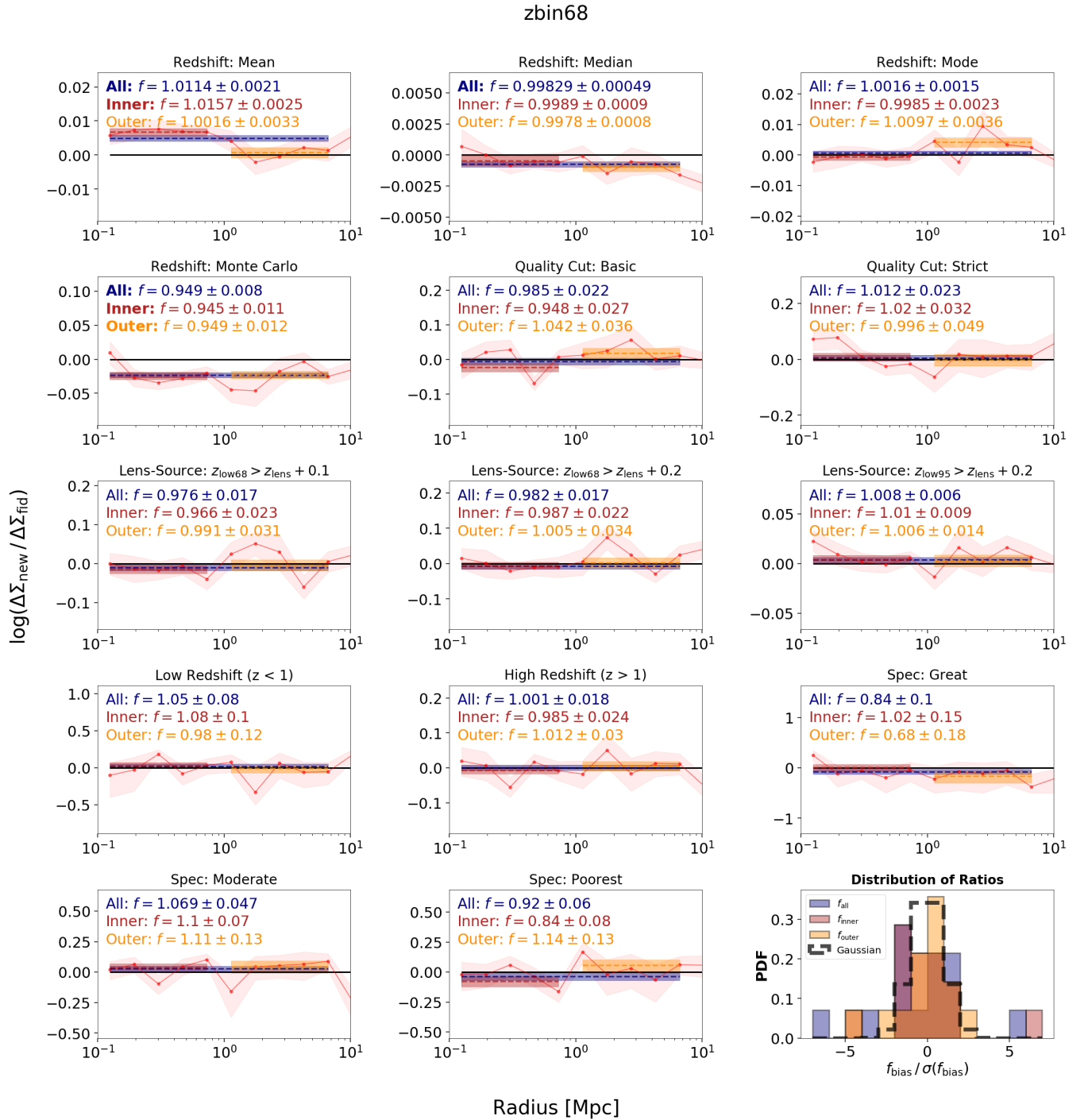
Figure 12. As Figure 10, but for zbin68 ( 0.6 < z_{\text{lens}} \leq 0.8 ).
