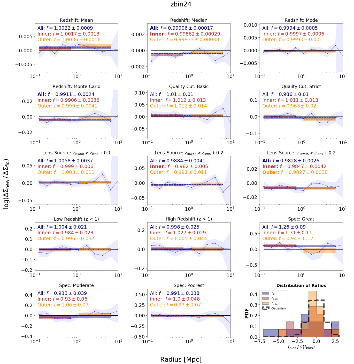
Figure 10. Bootstrap ratios f_{\text{new, fid}} between new \Delta\Sigma_{\text{new}}(R) signals computed using the zbin24 lens sample ( 0.2 < z_{\text{lens}} \leq 0.4 ) relative to our fiducial sample \Delta\Sigma_{\text{fid}}(R) . The null result ( f = 1 ) is shown as a solid black line, while the maximum-likelihood estimator for f_{\text{all}} (dark blue) and f_{\text{inner}} and f_{\text{outer}} (dark red) for each sample are shown as dotted lines and listed in the upper-left-hand corner of each plot. 1\text{-}\sigma errors on all quantities are shown as shaded regions. A 1-D histogram of the error-normalized distribution of f , f_{\text{inner}} , and f_{\text{outer}} is displayed in the bottom-right corner along with a Gaussian distribution for reference. Most of the computed ratios are consistent with the expected null result at 3\sigma ; those that disagree are highlighted in bold. Although these disagreements are statistically significant, some (e.g., with respect to z_{\text{med}} ) are negligible in practice since their impact is \lesssim 1\% . In general, f_{\text{outer}} is more unbiased for all samples than f and f_{\text{inner}} . See §7 for additional discussion and details.
