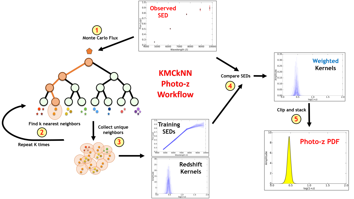
Figure 5. A schematic outline of the major steps in our KMCKNN based algorithm described in §4.3. First, a Monte Carlo realization of the target object indexed by g is matched with a set of k nearest neighbors based on a Monte Carlo realization of all training objects indexed by h . After repeating this procedure K times, all unique neighbors in the training set are identified and the corresponding photometric posteriors P(h|g) are computed. These are then used to derive a photo- z PDF based on a posterior-weighted mixture of the corresponding redshift kernels P(z|h) .
