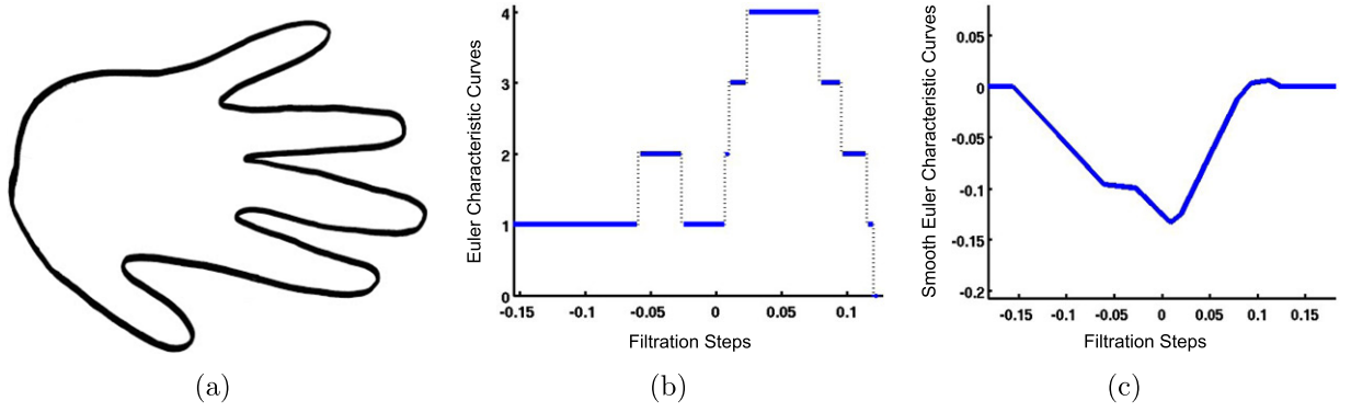
Figure 2. Example illustrating the evolutionary tracking of topological features for a given shape. (a) A two-dimensional contour of a hand, for which the Euler characteristic (EC) is calculated and tracked with respect to a horizontal filtration. (b) The Euler characteristic curve of the two-dimensional contour. At the leftmost filtration level on the x -axis, the EC value is equal to 1 on the y -axis. This indicates one connected component corresponding to the thumb in the hand. Just before level -0.05 , the index finger appears, which increases the value of the EC to 2. (c) The corresponding smooth Euler characteristic (SEC) curve. This found by taking the mean value of the EC curve in (b), subtracting it from every point along the x -axis, and integrating over the range of extremal heights (see Section 2.3). Since there are no holes in a hand, the EC reduces to the sum of connected components as they appear with the filtration. A version of this figure has been previously published (Turner, Mukherjee, and Boyer 2014).
