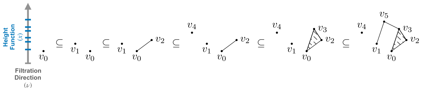
Figure 1. Demonstrating a filtration by height (as a function of x ) in the vertical direction v of a simplicial complex K . The inclusions ( \subseteq ; from left to right) indicate the evolution of K with the filtration depicted by the hash marks (from the bottom to top) on the y -axis, where each element (i.e., vertex, edge, and face) is included at its maximal height x in the vertical direction v , as given in Equation (1) from Section 2.3. Starting from the lefthand side, the vertex v_0 is first added and it remains present in each subsequent inclusion, while the vertex v_1 emerges during the second inclusion and then remains. Similarly, the edge v_0v_2 connecting vertices v_0 and v_2 appears at the third inclusion, and the face \langle v_0v_2v_3 \rangle forms at the fourth. Altogether, according to these inclusions, the collection of vertices in K are shown to evolve as follows: (i) \langle v_0 \rangle ; (ii) \langle v_0, v_1 \rangle ; (iii) \langle v_0, v_1, v_2 \rangle ; (iv) \langle v_0, v_1, v_2, v_4 \rangle ; (v) \langle v_0, v_1, v_2, v_3, v_4 \rangle ; and at the final inclusion, (vi) \langle v_0, v_1, v_2, v_3, v_4, v_5 \rangle . Similarly, the collection of edges in K evolves as follows: \langle v_0v_2 \rangle appears at the third, \langle v_0v_2, v_0v_3, v_2v_3 \rangle emerges at the fifth; and \langle v_0v_2, v_0v_3, v_2v_3, v_1v_5, v_3v_5 \rangle forms at the final inclusion. This evolution of vertices, edges, and faces forms (persistence) vector spaces of i -chains, and may be written as such for concise notation (see the supplementary materials for further details). A version of this figure has been previously published (Turner, Mukherjee, and Boyer 2014).
