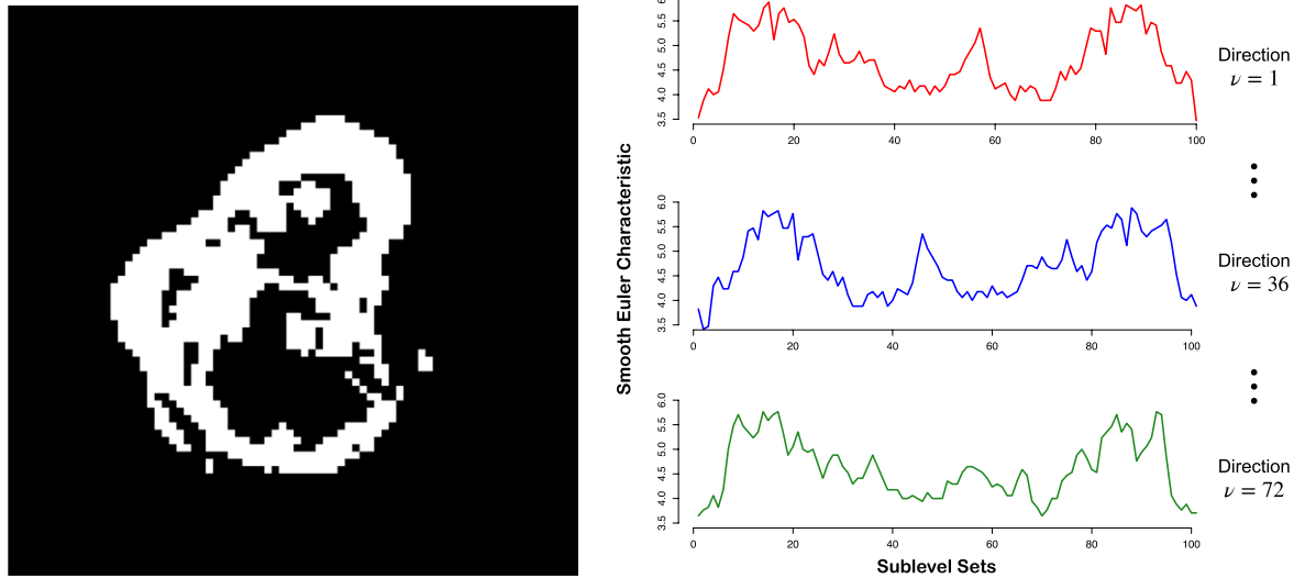
Figure 3. Example of a segmented tumor (on the left) with its corresponding SECT curves (on the right). On the right side, we illustrate the curves for directions \nu = 1 , 36, and 72, respectively. The x-axis shows the number of sublevel sets (i.e., steps) as the filtration progresses, which we fix to be 100 per slice. In the radiomic prediction analysis, all 72 curves are concatenated together to create a 7200-dimensional covariate vector for the patient.
