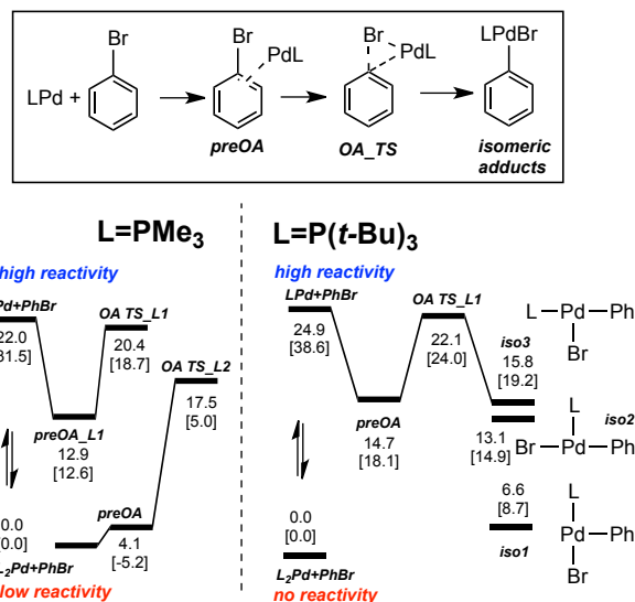
Figure 1. Oxidative addition of PhBr to trimethyl phosphine and tri- tert -butyl phosphine ligated Pd. Free energies and enthalpies (in brackets) are in kcal/mol. Here and further, unless specified otherwise, the values are computed using rM06/6-311+G(d,p), Pd, Br: LANL2DZ, SMD: toluene // rB3LYP/6-31G(d), Pd, Br: LANL2DZ.
