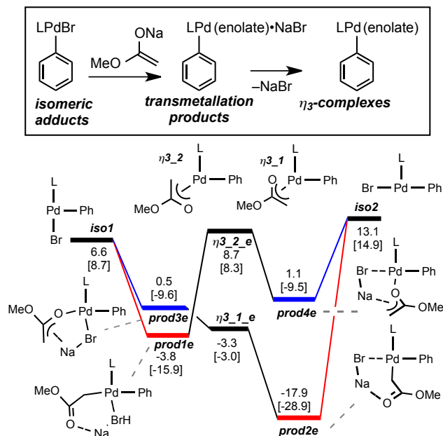
Figure 5. Transmetalation adducts and isomeric \eta^3 -Pd complexes resulting from the carbon (red) or oxygen (blue) attacks by the ester enolate
