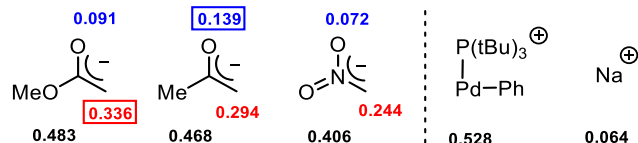
Figure 7. Global (in black) and local (blue for oxygen and red for carbon) softness parameters, eV -1 . Values computed using rB3LYP/6-311+G(d,p), Pd, Br: LANL2DZ, IEFPCM: toluene. Global softness was calculated as an inverse of hardness 9 : S = 1/\eta . In turn, global hardness was calculated from MO data using finite differences
