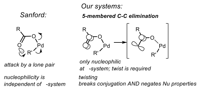
Figure 9. Orientation of orbitals for 5-membered reductive elimination transition states.
