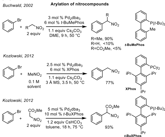
Scheme 1. (A) Typical reaction conditions for arylation of ketones and esters. (B) Examples of conditions for arylation of different types of nitro compounds
