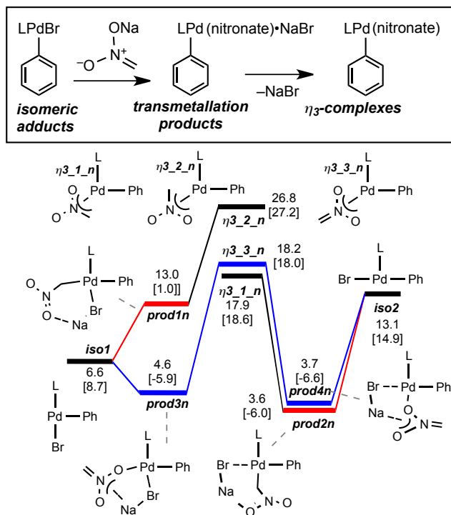
Figure 6. Transmetallation adducts and isomeric \eta^3 -Pd complexes resulting from the carbon (red) or oxygen (blue) attacks by the nitronate on the isomers of P(t\text{-Bu})_3\text{PdPhBr} . Free energies and enthalpies (in brackets) are in kcal/mol.
