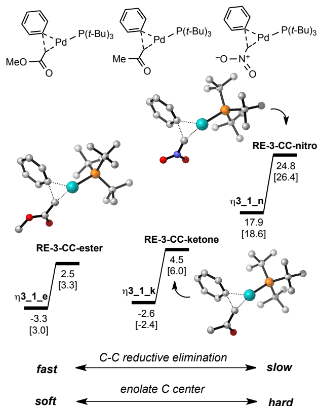
Figure 10. Energy profiles for C-C reductive elimination transition states. L = P( t -Bu) 3 . Free energies and enthalpies (in brackets) are in kcal/mol.
