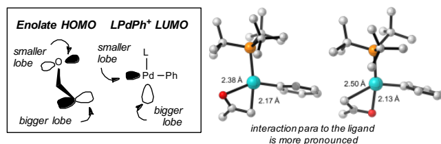
Figure 4. Left: HOMO of the enolate fragment and LUMO of the \text{LPdPh}^+ . Right: structures of the \eta^3 Pd complexes resulting from reaction with the ketone enolate.
