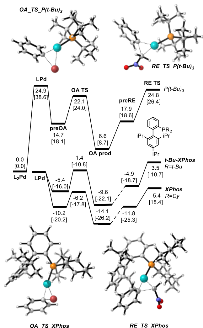
Figure 12. Energy profiles for the \alpha -arylation of nitromethane using P(tBu)_3 , XPhos and t -Bu-XPhos ligands. In calculations we used model ligands where para -isopropyl group on the bottom ring is permuted to hydrogen. Free energies and enthalpies (in brackets) are in kcal/mol.
