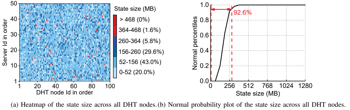
Figure 10: The load balance evaluation of FP4S for a collection of concurrently running stream applications.
