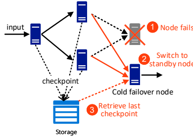
Figure 3: The checkpointing recovery workflow.
