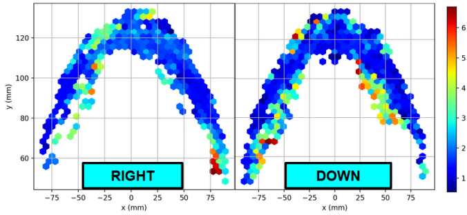
Fig. 5. Heatmap illustrations of the critic (for the simulated hand) error values projected on the x-y plane with regards to different action directions.
