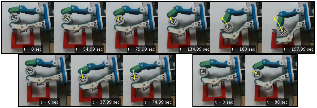
Fig. 6. Snapshots of the real hand experiments to manipulate the cylinder into the red horseshoe: roll-outs of (top) successful H-CRITIC planned path, (bottom left) standard planned path that collided and (bottom right) standard planned path that reached overload of the actuators.
