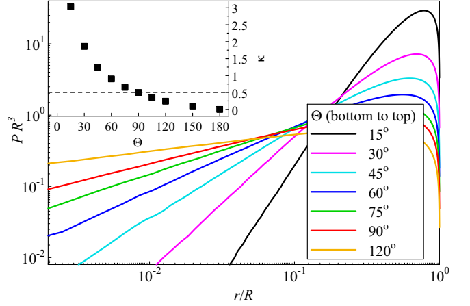
FIG. 18. Scaled stationary probability density PR^3 of FBM with \alpha = 0.8 in a spherical cone with outer radius R = 10^3 for various opening angles \Theta . The graphs show PR^3 on the symmetry line of the cone as functions of r/R . ( 10^6 particles performing 2^{25} time steps.) Inset: Exponent \kappa , determined from power-law fits, P(r) \sim r^\kappa , of the data close to the center ( r/R \ll 1 ) vs. opening angle \Theta . The dashed line marks the value 2/\alpha - 2 = 0.5 .
