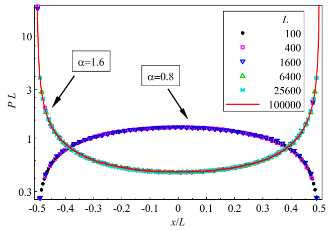
FIG. 3. Scaling plot of the stationary probability density showing PL vs. x/L for \alpha = 1.6 and \alpha = 0.8 for several interval length L . Each distribution is based on 10^4 to 10^5 particles; P is averaged over a number of time steps after a stationary state has been reached.
