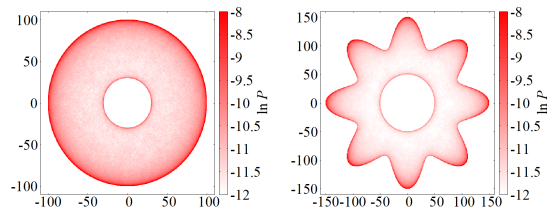
FIG. 10. Heat maps of the stationary probability density P for \alpha = 1.6 , computed from 100 particles performing up to 2^{21} time steps.
