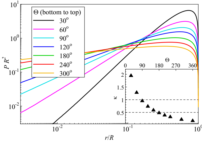
FIG. 15. Scaled stationary probability density PR^2 of FBM with \alpha = 0.8 on a circular sector with outer radius R = 10^3 for various opening angles \Theta . The graphs show PR^2 on the symmetry line of the sector as a function of the scaled distance r/R from the center of curvature. ( 10^6 particles performing 2^{25} time steps.) Inset: Exponent \kappa , extracted from power-law fits, P(r) \sim r^\kappa , of the PDF close to the center ( r/R \ll 1 ) vs. opening angle \Theta . The dashed lines mark the values 2/\alpha - 2 = 0.5 and 4/\alpha - 4 = 1.0 .
