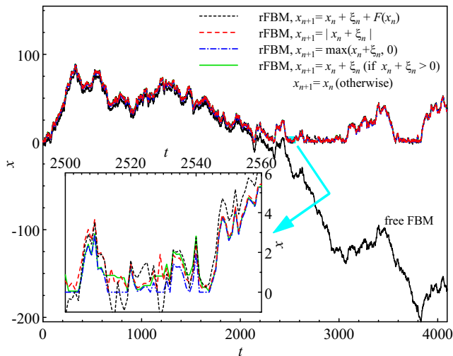
FIG. 5. Example trajectories of FBM ( \alpha = 1.2 ) with a reflecting wall at the origin (rFBM), implemented via the boundary conditions (8), (9), (10), and (11). For the soft wall (11), the force parameters are F_0 = 0.5 and \lambda = 1 . The free FBM trajectory is shown for comparison. Inset: Zoomed-in view of the trajectories very close to the wall.
