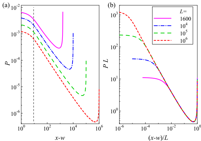
FIG. 7. (a) Stationary probability density P vs. distance x-w from the wall for \alpha = 1.6 , and several interval lengths. The walls are implemented as repulsive forces (12) with F_0 = 0.2 and \lambda = 0.2 . The dashed line marks the widths of the wall region. (b) The same data plotted in scaled variables PL vs. (x-w)/L .
