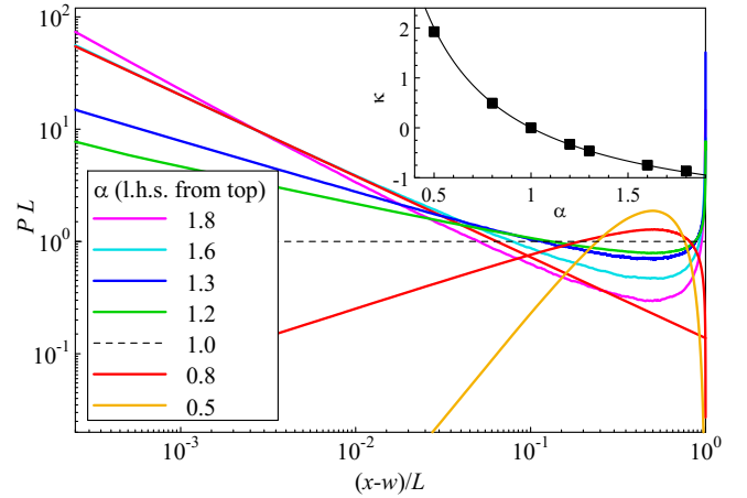
FIG. 4. Scaled stationary probability density PL vs. scaled distance (x - w)/L from the wall for several \alpha . The system sizes range from L = 200 for \alpha = 0.5 to L = 10^6 for the largest \alpha . Each distribution is based on 10^4 to 10^5 particles; P is averaged over a large number (up to 2^{25} ) of time steps after a stationary state has been reached. Inset: Exponent \kappa extracted from power-law fits of P(x) close to the wall. The solid line is the conjecture \kappa = 2/\alpha - 2 .
