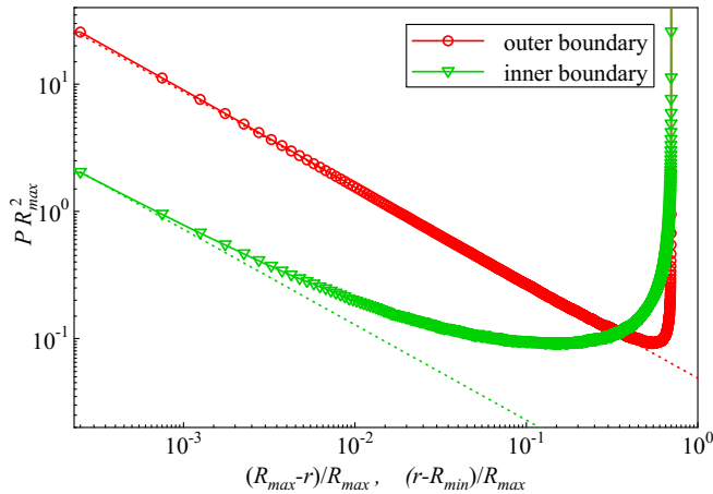
FIG. 12. Scaled stationary probability density on a ring with outer radius R_{max} = 10^6 and inner radius R_{min} = 0.3R_{max} vs. scaled distance from both boundaries for \alpha = 1.6 . The simulations use 10^5 particles performing 2^{27} time steps. The dashed lines are fits to power laws with the conjectured exponent \kappa = 2/\alpha - 2 = -0.75 .
