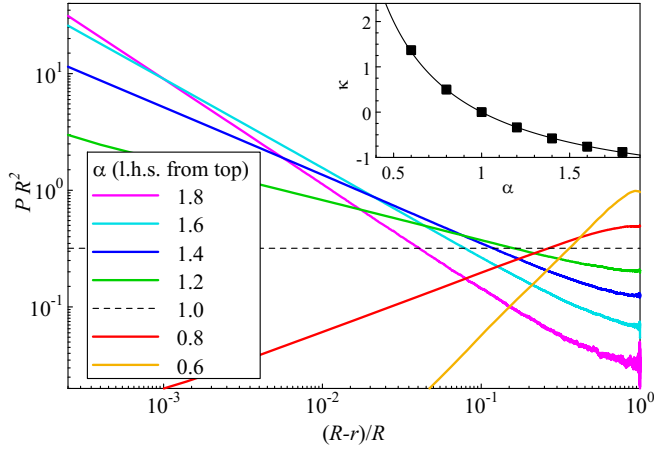
FIG. 11. Stationary probability density P(r) of FBM on circular domains (disks) of radius R for several \alpha . The data are plotted as PR^2 vs. scaled distance (R - r)/R from the wall. System sizes range from R = 10^6 for \alpha = 1.8 to R = 1000 for \alpha = 0.6 ; the simulations use 10^4 to 10^5 particles and up to 2^{29} time steps. Inset: Exponent \kappa extracted from power-law fits of P(r) close to the wall. The solid line is the one-dimensional conjecture \kappa = 2/\alpha - 2 .
