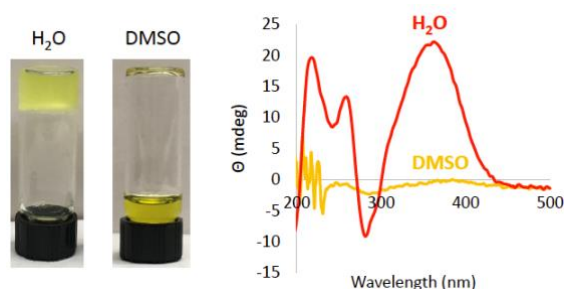
Fig. 4: Photographs of a hydrogel made from 8-disulfideG 1 (0.5 wt%, 8 mM) and a solution of 8-disulfideG 1 (8 mM) in DMSO. The red curve shows CD spectrum of hydrogel made from 8-disulfideG 1 (0.5 wt%, 8 mM) and the yellow curve shows a CD spectrum of a solution of 1 (8 mM) in DMSO.
