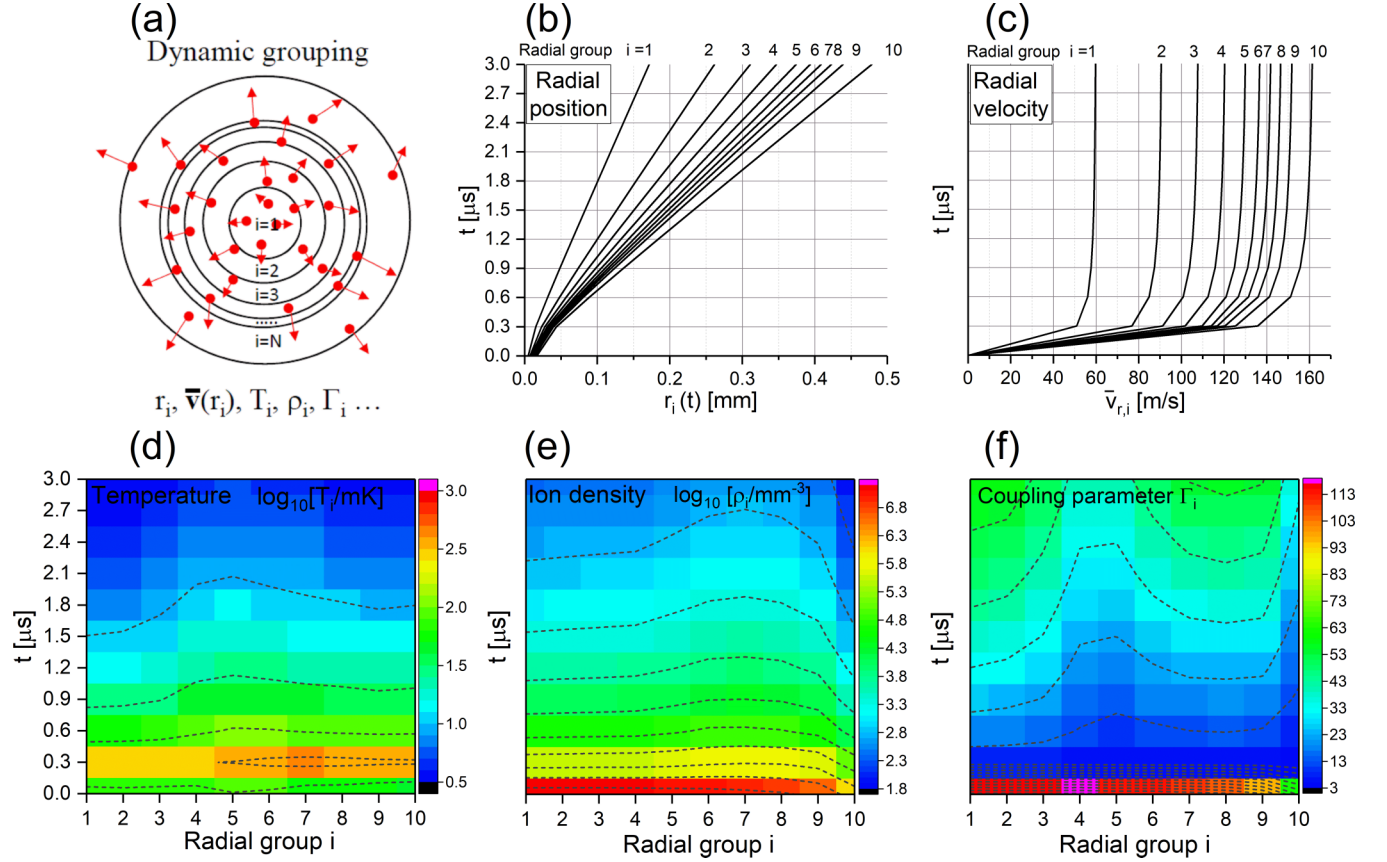
FIG. 4. (a) Sketch of the radial-partition (shell) model explained in the text. The shell radii, the macroscopic velocity \bar{v}_{r,i}(r, t) , and other plasma parameters depend on shell index i and time. (b) Average shell radii (horizontal axis) obtained for 125 ions with an initial cloud radius of about 20 \mu\text{m} vs expansion time (vertical axis). The shell indices are listed on top. (c) Corresponding average shell velocities. (d) Temperature vs shell index (horizontal axis) and time (vertical axis), displayed on a logarithmic color map. (e) Ion density vs shell index (horizontal axis) and expansion time (vertical axis), displayed on a logarithmic color map. (f) Coulomb coupling parameter \Gamma vs shell index (horizontal axis) and time (vertical axis), displayed on a linear color map.
