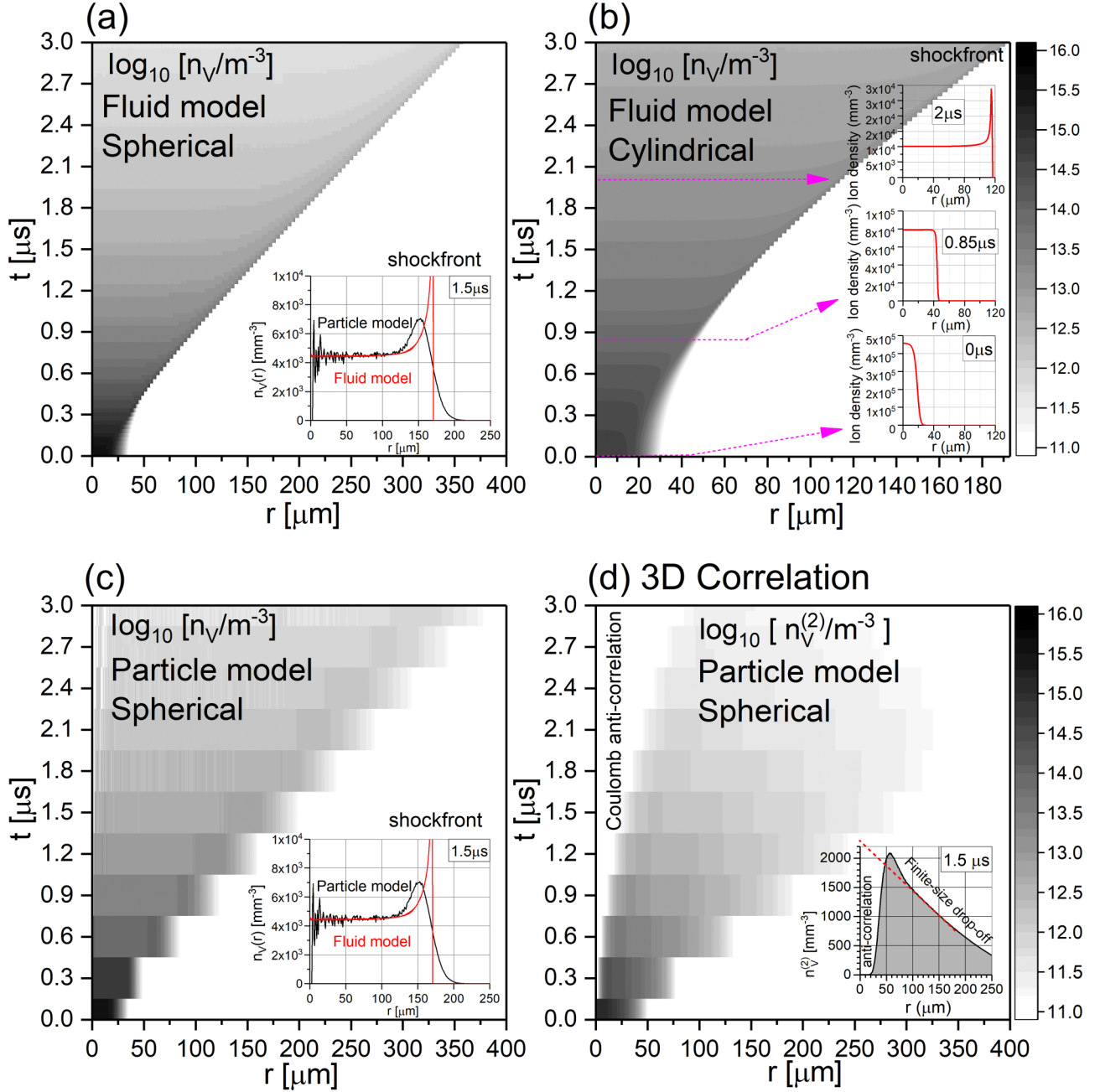
FIG. 6. Density maps vs radius r (horizontal axes) and expansion time t (vertical axes) from fluid-model simulations of the expansion of (a) a spherical and (b) an infinitely long cylindrical plasma, with radial profiles at selected times shown in the insets. (c) A molecular dynamics simulation with parameters as in (a). The insets in (a)–(c) for t \geq 1.5 \mu s show shock-front singularities. The molecular dynamics simulation reveals that the plasma microfields broaden the shock fronts and reduce their contrast. (d) A molecular dynamics simulation of the density correlation function, n_V^{(2)}(r, t) , vs correlation distance r and expansion time t . The inset shows n_V^{(2)}(r, t) at t = 1.5 \mu s , with a trend line (red dashed line) that visualizes the overall drop due to the finite size of the plasma.
