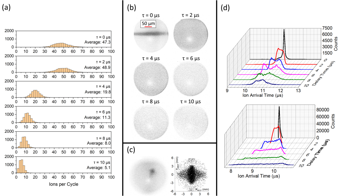
FIG. 2. (a) Histograms of ion counts per cycle for the indicated expansion times \tau . (b) Averaged pictures of the plasma images on the MCP plane for the indicated expansion times. The distance scale in the upper-left image corresponds to the distance in the object plane. The light spot is an area of reduced ion detection rate; its origin is under investigation. (c) Experimental (left) and computational (right) MCP images of plasma at \tau = 10 \mu\text{s} in the presence of a quadrupole electric field. Instead of expanding outwards and leaving the field of view, the ions are refocused by the electric field and accumulate at a plasma focus, which maps onto a localized region on the MCP with well-above-average count density. (d) Experimental (top) and computational (bottom) distributions of ion MCP arrival times (horizontal axis) for different plasma expansion times (tilted axis). To enhance visibility, the count axes for the experimental data are magnified by factors of 1, 2, 4, 8, and 8, in ascending order of expansion times. Likewise, the count axes for the computational data are magnified by factors of 1, 8, 32, 64, 64, and 64.
