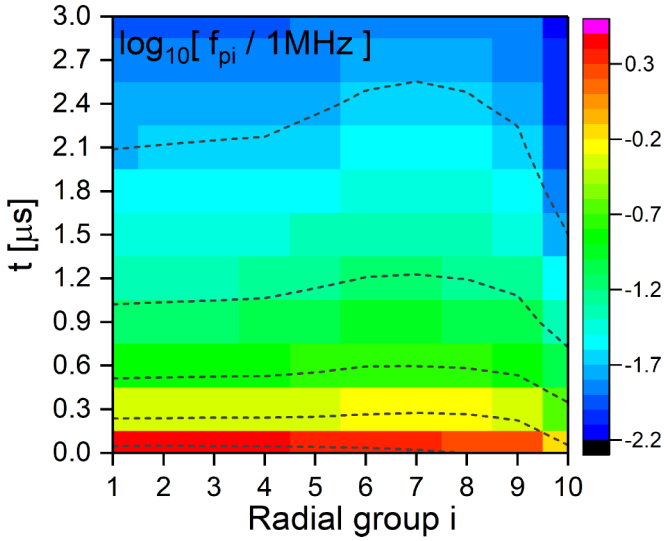
FIG. 5. Ion-plasma frequency f_{p,i} from the same simulation as in Fig. 4 vs shell index (horizontal axis) and expansion time (vertical axis), displayed on a logarithmic color map.
