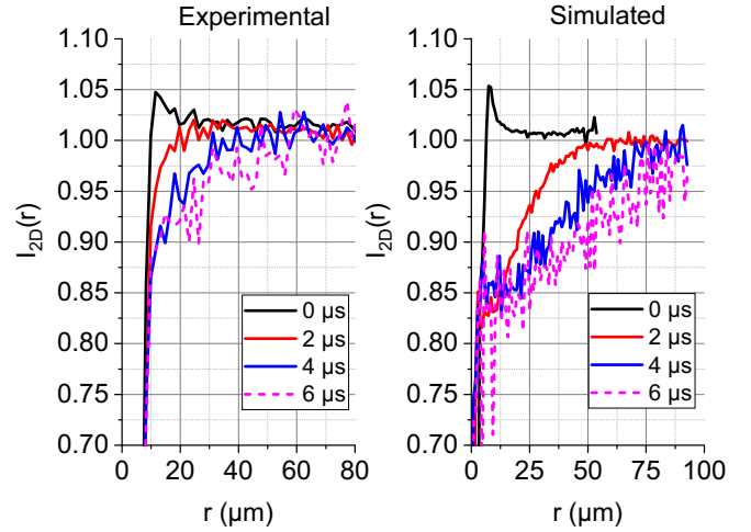
FIG. 3. Projected, two-dimensional ion pair correlations I_{2D}(r) for the indicated expansion times, measured vs the radial coordinate in the xz object plane. The left panel is for experimental data and the right one for simulated data. Pair correlations for \tau > 6 \mu\text{s} are not shown because they are too noisy, as a result of the diminishing ion number in the images. The steep drop in the data at distances \lesssim 8 \mu\text{m} is an experimental artifact caused by the finite blip size of the ion counts on the MCP.
