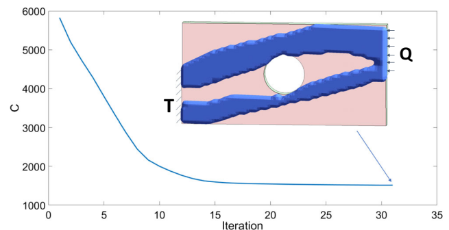
Fig. 7 Topology and convergence plot for plate problem
