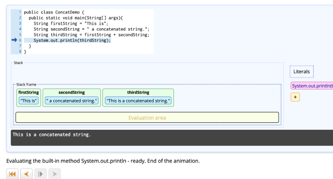
Figure 2: Animation of String concatenation in Java.
