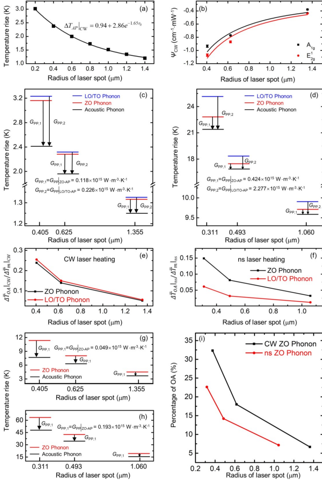
Figure 7. Determination of coupling factors of MX 2 (MoS 2 and MoSe 2 ) under CW and ns laser heating. (a) Theoretical temperature rise of acoustic phonons in MoS 2 under CW laser heating. (b) \psi_{CW} against laser spot size for MoS 2 . (c-d) Distinguished temperatures of LO/TO phonon, ZO phonon, and AP under
