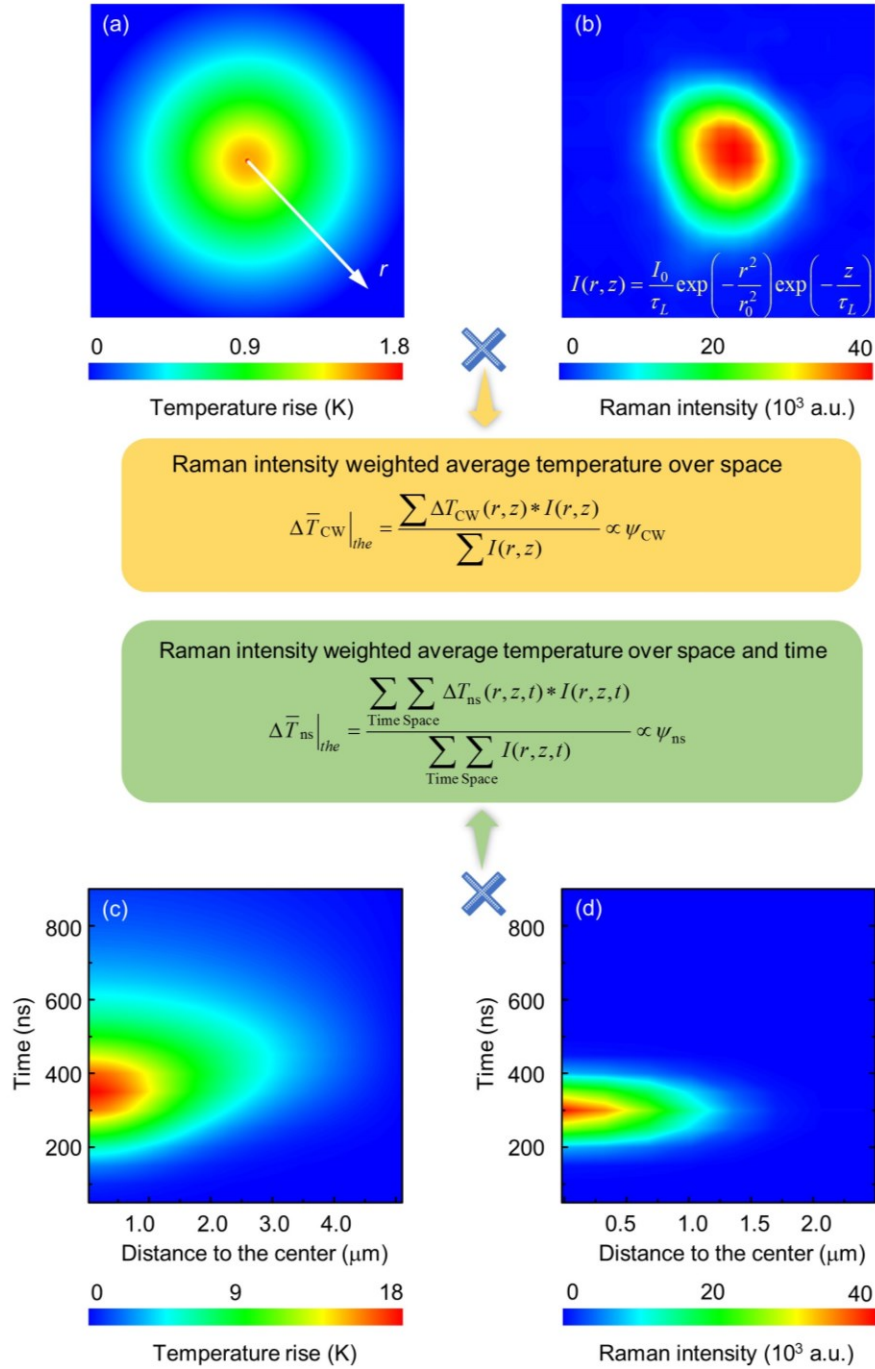
Figure 5. Physics of the measured temperature rise in ns ET-Raman. (a) Temperature distribution under CW laser heating. (b) Raman intensity distribution of CW laser in space. (c) Temperature map in the time-space domain under ns laser heating. (d) Raman intensity distribution of ns laser in time and space domains. The measured temperature rise is Raman intensity weighted over space domain in CW laser heating, and over time and space domains in ns laser heating. These two are proportional to the \psi values obtained in the ns ET-Raman experiments. All these are considered in our 3D numerical modeling.
