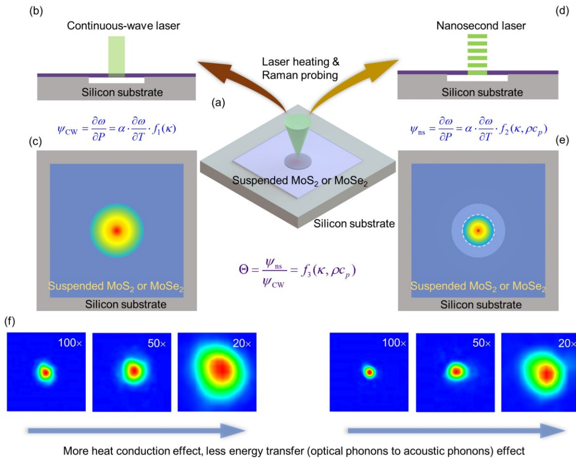
Figure 2. Physical concept of the ns ET-Raman technique. (a) \text{MoS}_2 or \text{MoSe}_2 nanosheets are transferred onto the silicon substrate with a hole beneath. A CW laser and an ns laser with the same wavelength (532 nm) are used to generate two energy transport states in the time domain [(b) and (d)]. The laser is used for both heating the sample and probing the Raman signal. (c) and (e) Heating effect of CW laser and ns laser. Based on the different contribution of in-plane thermal conductivity under the two energy transport states, the in-plane thermal conductivity of the sample could be obtained. (f) With the increase of laser spot size, the effect of energy transfer from optical phonons to acoustic phonons decreases. The size of all the panes in (f) is 4.9 \mu\text{m} \times 4.9 \mu\text{m} .
