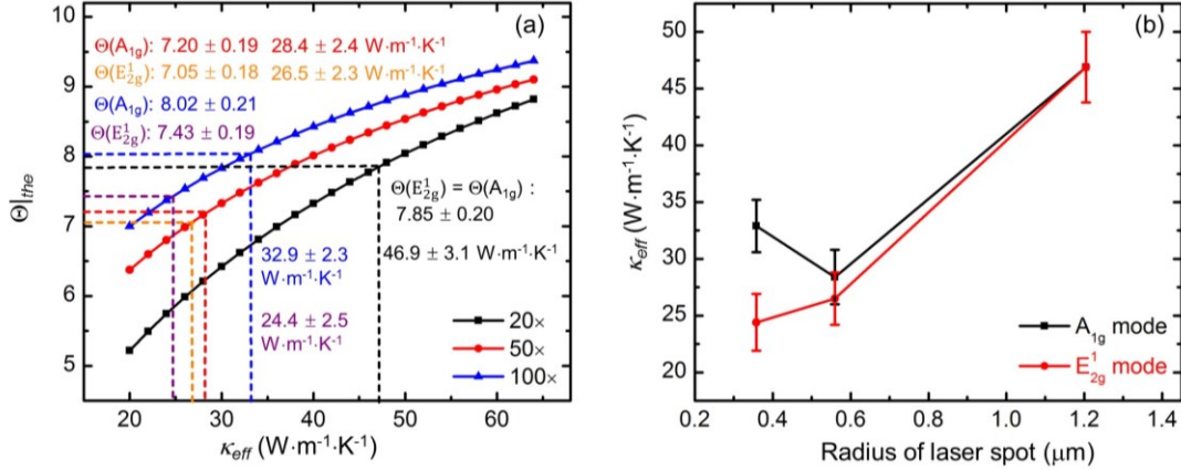
Figure 6. 3D numerical modeling and data processing results for the 55 nm thick MoS 2 . The in-plane \kappa_{eff} is obtained by interpolating the experimental results in the curves. (a) In-plane \kappa_{eff} obtained under the 20×, 50×, and 100× objective lenses for the two Raman modes. (b) In-plane \kappa_{eff} variation against laser spot size of the two Raman modes.
