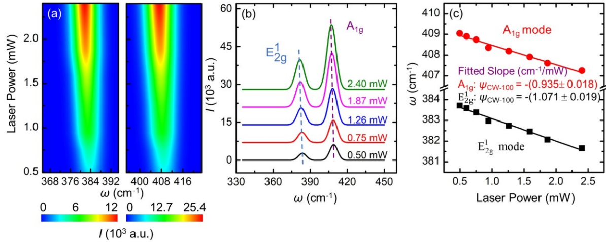
Figure 4. (a) 2D contour map of MoS 2 Raman peaks. This figure demonstrates the variation of Raman shift against the laser power of CW laser with 100 \times objective lens. (b) Five representative Raman spectra of MoS 2 with increased laser power of CW laser with 100 \times objective lens. Both modes are redshifted with increased laser power. For CW laser with 100 \times objective lens, the Raman shifts of the two modes as a function of laser power are shown in (c).
