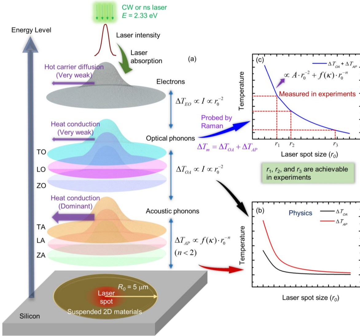
Figure 1. Illustration of the cascading energy transfer process among different energy carriers in 2D materials. (a) A continuous-wave (CW) or a nanosecond (ns) laser irradiates the suspended 2D material. With the laser absorption, the energy is transferred to electrons first. Then, the energy is mainly transferred from electrons to optical phonons. Next the optical phonons will transfer most of the energy to acoustic phonons. Finally, the energy will be transferred to the whole area of the sample through heat conduction. (b) The temperature difference between optical phonons and acoustic phonons decreases ( \sim r_0^{-2} ) against increased laser spot size ( r_0 ). The temperature difference between acoustic phonons and environment also decreases with the increased laser spot size, but with a different rate. (c) The thermal conductivity of the sample and the energy coupling coefficient between optical phonons and acoustic phonons can be determined by using three achievable laser spots in experiments ( r_i , i=1, 2, 3 ). Note the temperature mentioned in the figures is a value at a point within the laser heating area for ease of physics discussion. In Raman experiment, the measured temperature is a Raman intensity-weighted average, and is considered in our modeling and data processing.
