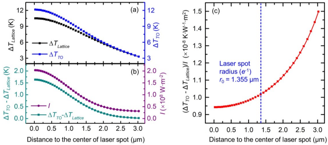
Figure 8. (a) Temperature rise variation of TO phonons and lattice in space under CW laser irradiation. (b) Variation of temperature rise difference between TO phonons and lattice in space. (c) Ratio of temperature rise difference over laser intensity.
