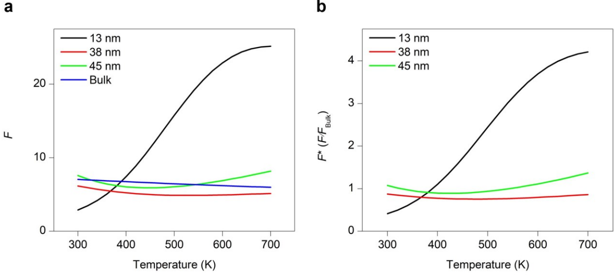
Figure 9. (a) Raman intensity enhancement factor ( F ) as the function of T . This plot includes the effects of both optical properties evolution and thermal expansion at higher temperatures. (b) F^* shows the normalized F with respect to F_{\text{Bulk}} . Note that spacing ( t_2 ) values that are used in this calculation are based on theoretical values [Figure 8(a)], which are obviously not consistent with the experimental \text{In}^* , as shown in Figure 6(b).
