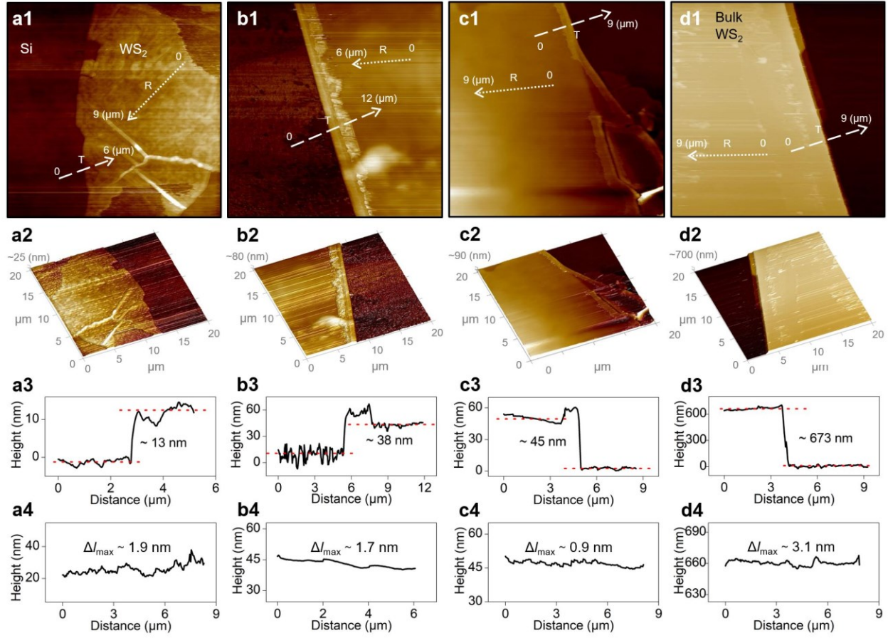
Figure 1. AFM imaging of the four supported \text{WS}_2 samples. (a1-d1) 2D AFM images of all samples. (a2-d2) 3D AFM images of all samples. (a3-d3) Thickness profile of the samples that correlates to the white dashed arrows (labeled by T). (a4-d4) Roughness profile on the surface of \text{WS}_2 that corresponds to the white dotted arrows (labeled by R). These dotted arrows cover the location of laser spot.
