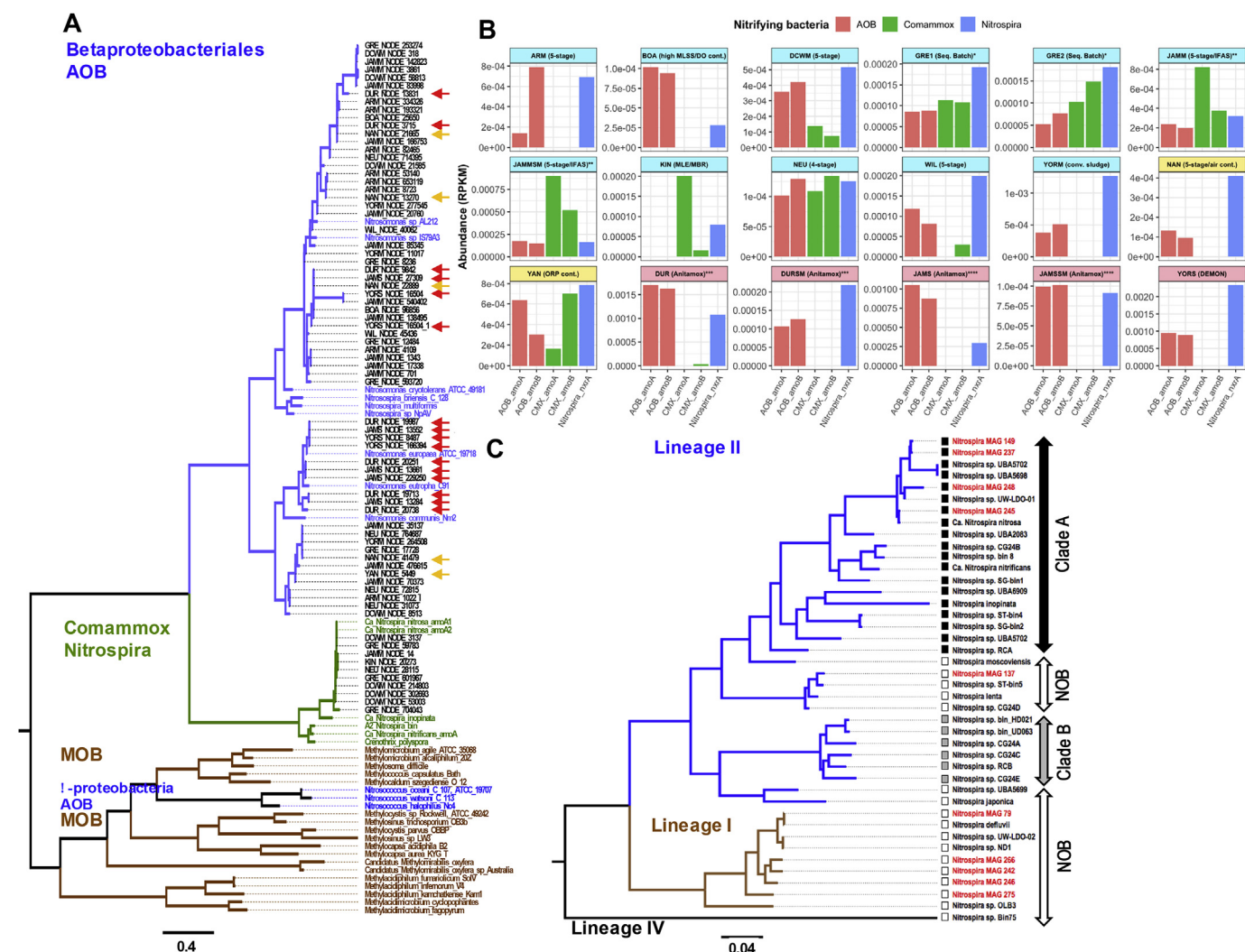
Fig. 3. Maximum likelihood phylogenetic tree of amoA gene sequences recovered from gene centric de novo assembly along with reference amoA and pmoA gene sequences. Clades are colored by functional grouping and labels for reference sequences within each cluster are colored according to the functional group, while amoA sequences recovered from this study are shown in black labels. Red arrows and orange diamonds indicate amoA gene sequences recovered from PNA and SND systems respectively, while those recovered from ND systems are not annotated. amoA gene sequences from YAN and KIN are not shown in the phylogenetic tree due to recovery of short sequences not suitable for tree construction. (B) Abundance (RPKM) of amoA , amoB gene sequences of AOB and comammox bacteria, and nrrA gene sequences of Nitrospira are shown. (C) Phylogenetic placement of Nitrospira MAGs (red label) with 32 reference genomes (black label). Clade A (black squares), clade B (grey squares) comammox bacteria and canonical NOB (open squares). (For interpretation of the references to color in this figure legend, the reader is referred to the Web version of this article.)
