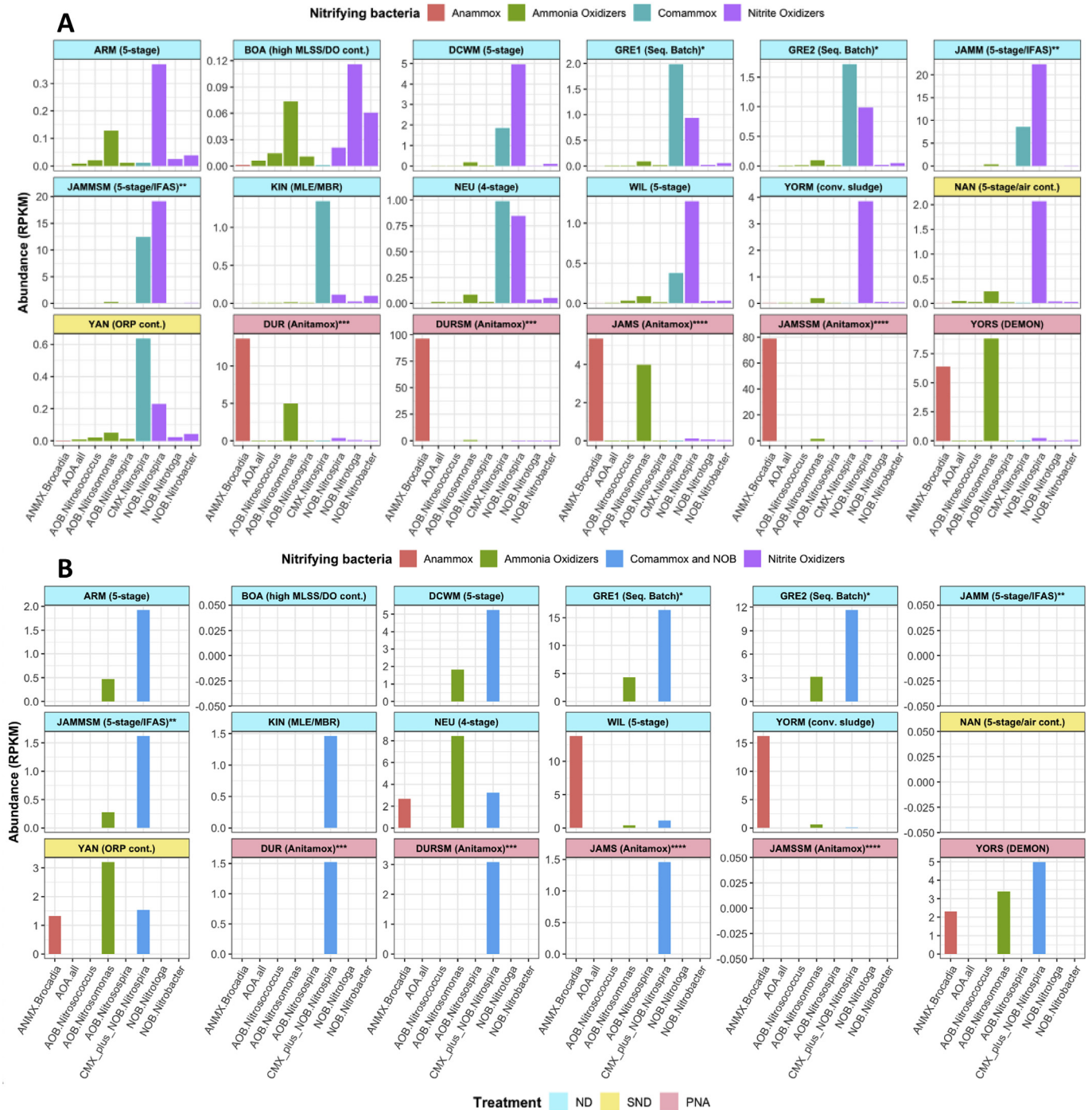
Fig. 2. Relative abundance of nitrifying organisms in nitrogen removal systems based on (A) mapping of reads to reference genomes and (B) classification of MATAM assembled 16S rRNA genes. Bar colors indicate type of nitrifying organism detected (see color legend below each figure), while facet color indicates process type (i.e., red: PNA, Blue: ND, and Yellow: SND). This information can also be found in Table 1. GRE1/GRE2* panels present abundance of nitrifying populations from two different reactors at the same treatment plant. JAMM/JAMMSM**, DUR/DURSM***, and JAMS/JAMSSM**** panels present abundance of nitrifying populations in the suspended phase and attached growth phase of the system, respectively. (For interpretation of the references to color in this figure legend, the reader is referred to the Web version of this article.)
