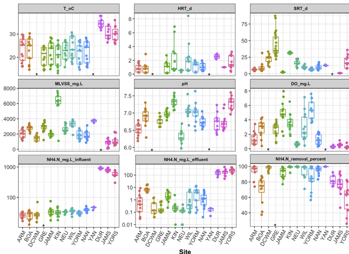
Fig. 1. Overview of key process parameters and performance metrics monitored as part of this study for 14 nitrogen removal systems. Column indicated with "" indicates lack of relevant process data for the respective nitrogen removal system.
