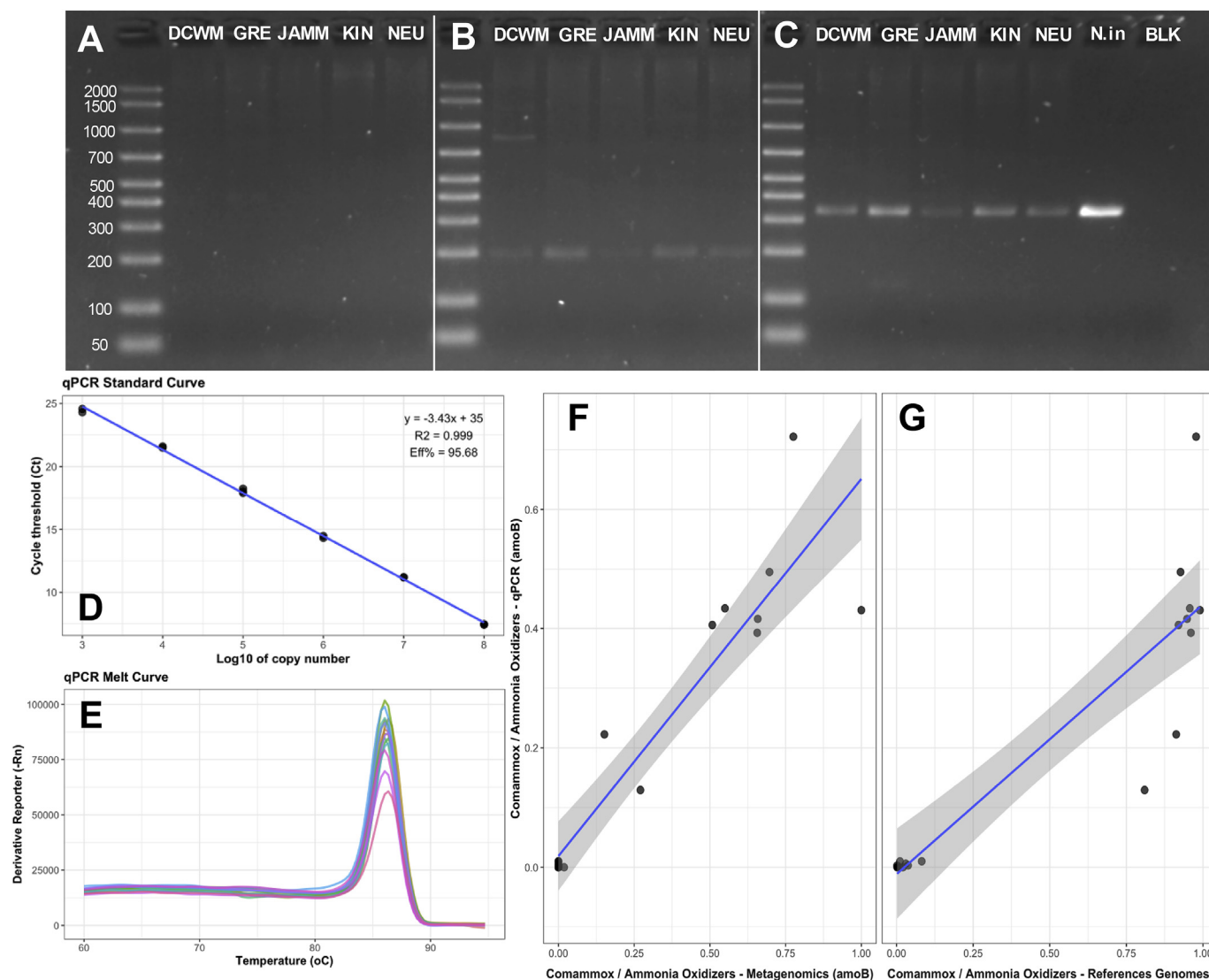
Fig. 4. Previously published primer sets for the amoA gene of comammox bacteria, i.e. (A) comaA , and (B) Ntspa-amoA , result in non-detection and unspecific amplification samples from DCWM, GRE, JAMM, KIN, NEU where comammox bacteria were detected using metagenomics. In contrast the newly designed amoB gene specific primers (C) result in a single band formation of the right size for these samples which is consistent with that amplified from Ca Nitrospira inopinata (N.in). BLK stands for PCR negative control. The primers exhibit excellent PCR efficiency (D), demonstrate clean melting curves (E), and provide estimates of comammox bacterial abundance consistent with those seen in PCR-free metagenomics analyses (F, G).
