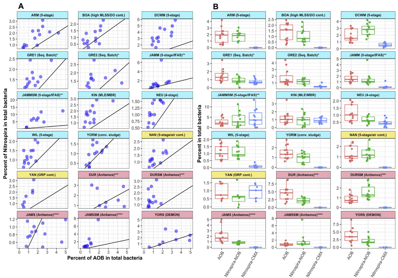
Fig. 5. (A) Comparison of the abundance of Nitrospira (% of total bacteria) to that of AOB (% of total bacteria) indicates that several systems with higher proportional abundance of Nitrospira when compared to the theoretical estimates (black line) if nitrification was being driven by AOB and NOB. (B) The abundance of AOB, Nitrospira -NOB, and comammox bacteria as a proportional of total bacterial abundance indicates that comammox bacteria were (1) consistently detected in systems with metagenomic evidence of their presence, (2) their abundance was lower than AOB in suspended growth systems where they were detected and high in systems with attached growth phase. Asterisks levels indicate samples from the same system.
