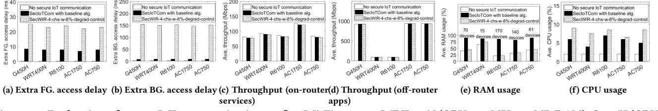
Figure 13: Evaluation of secure IoT communication on five Wi-Fi routers: WRT400N (CPU: 680MHz, 32MB RAM), G450H (CPU: 400MHz, 64MB RAM), AC750 (CPU: 580MHz, 64MB RAM), R6100 (CPU: 560MHz, 128MB RAM), and AC1750 (CPU: 720MHz, 128MB RAM).
