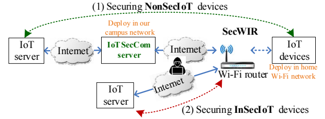
Figure 9: Experimental testbed.
