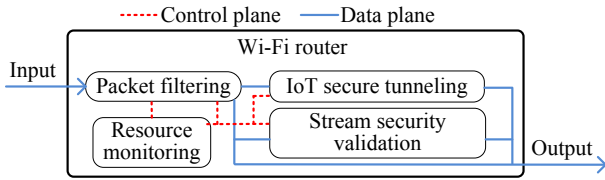
Figure 5: Architecture of SecWIR.
