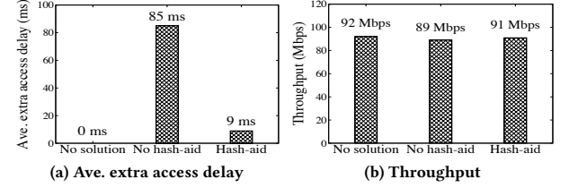
Figure 12: Evaluation of the stream security validation module on the Linksys WRT400N Wi-Fi router.
