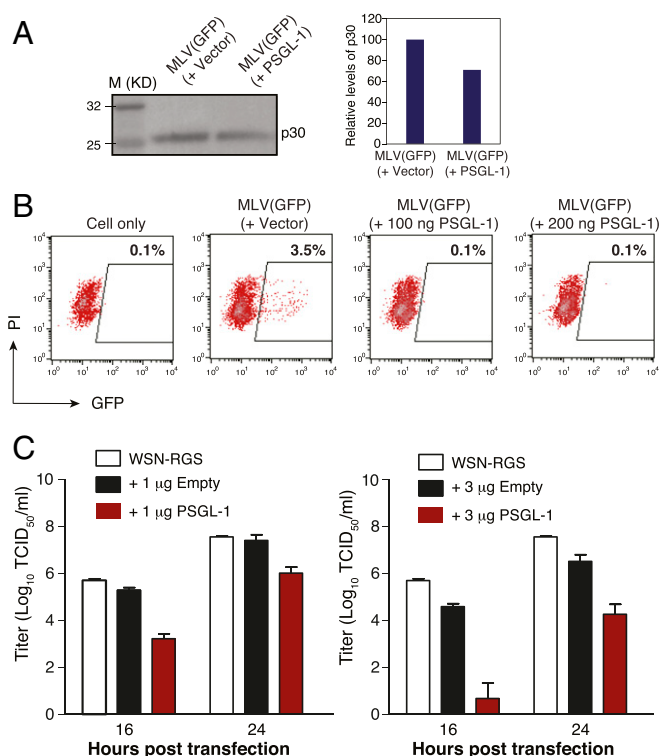
Fig. 5. PSGL-1 restricts MLV and influenza A virus infectivity. (A) HEK293T cells were cotransfected with an MLV helper vector, pSV- \psi -MLV-env + , pRetroQ-AcGFP-N1, pCMV-G, plus a PSGL-1 expression vector or an empty control vector. Virions were harvested and quantified by Western blot analysis using an anti-MLV p30 (CA) protein antibody. (B) MLV virions were harvested, and viral infectivity was quantified by infecting HEK293T cells and measuring GFP expression. (C) Eight vectors expressing each of the segments of the influenza A/WSN/33 (H1N1) genome were cotransfected with a PSGL-1 expression vector into HEK293T-MDCK cells. Viral particles were harvested at 16 and 24 h after cotransfection, and virion infectivity was quantified by a TCID 50 assay.
