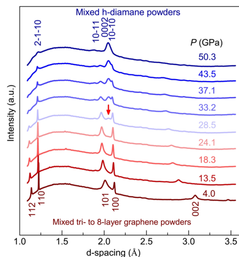
Figure 3. XRD results of mixed tri- to 8-layer graphene powders under compression indicating the structural transition to an atomically thin h-diamondlike structure at 28.5 GPa.
