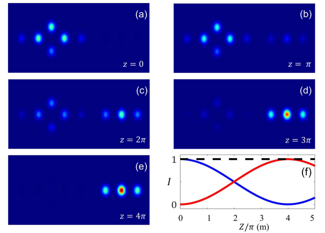
Fig. 4. Light propagation dynamics in a waveguide array formed by introducing a weak coupling between the main structure and its partner, as shown in (a)–(e). When mode ① of the main array is excited, we observe an efficient optical power transfer to the partner array after a propagation distance corresponding to z = 4\pi (in units of meter). On the other hand, if mode ② of the main array is excited, no appreciable power transfer to the partner array is observed (not shown here). The power transfer efficiency between the modes is illustrated in (f) where near perfect transfer is observed. The blue and red lines are the total power in the main and pattern arrays, respectively.
