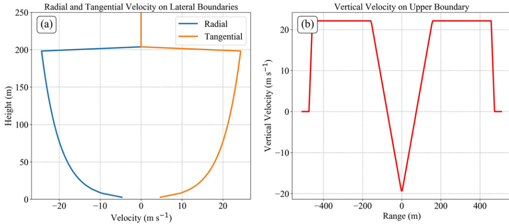
FIG. 1. (a) Profiles of radial velocity (blue) and tangential velocity (orange) on the lateral boundaries up to a height of 250 m AGL and (b) the vertical velocity profile (red) on the upper boundary to a range of 450 m.
