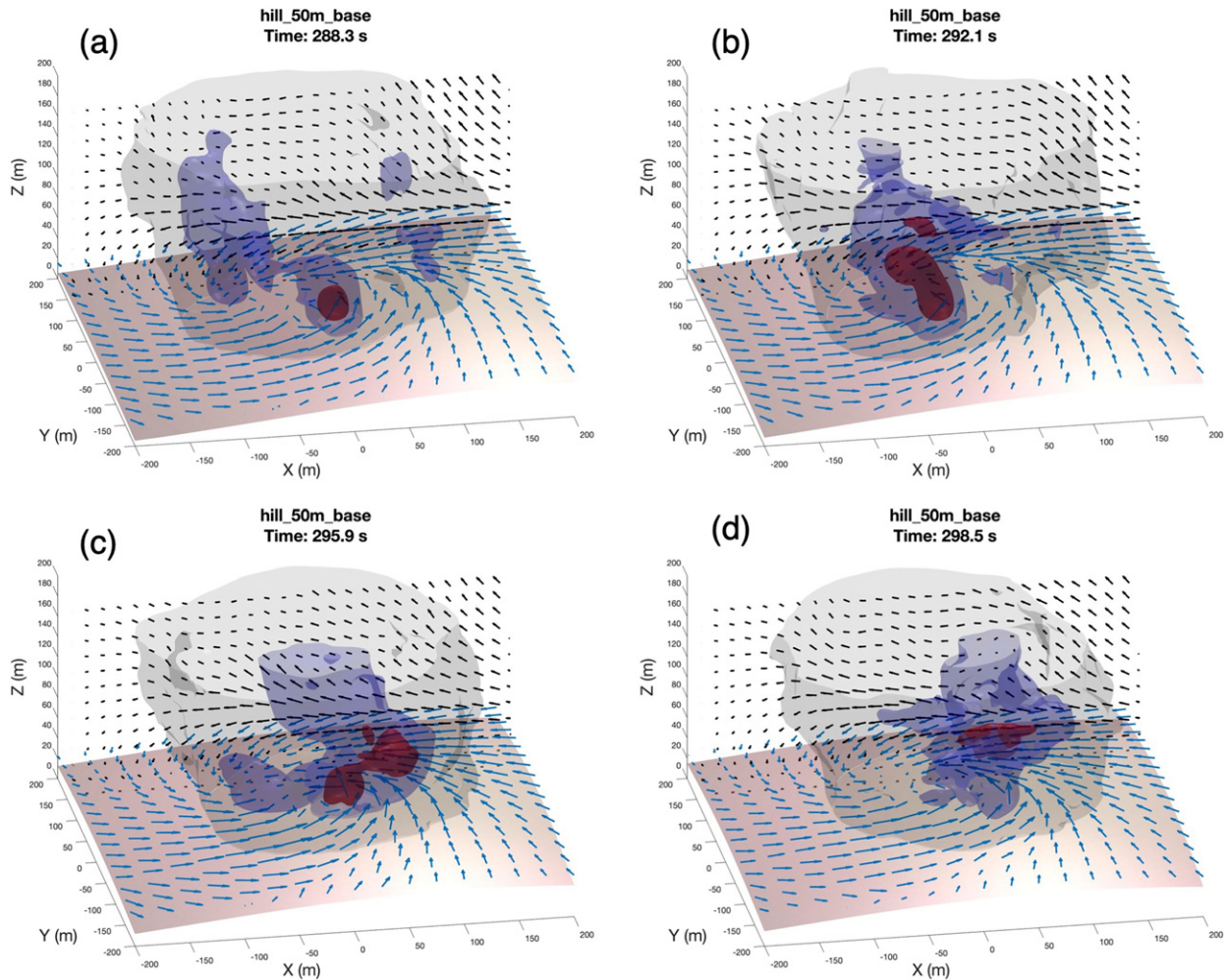
FIG. 9. Sequence of images depicting subvortex behavior corresponding to the same times as Fig. 8. Shaded contours and arrows are as in Fig. 4. Terrain height is represented by the shaded lower boundary where darker pink surfaces are lower terrain and brighter yellow/white surfaces are higher terrain.
