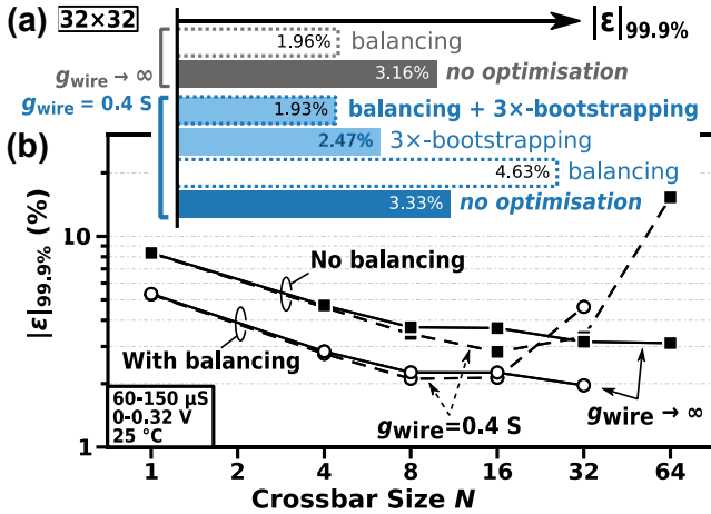
Fig. 8. Worst-case error for (a) 32 \times 32 crossbar circuit and (b) as a function of crossbar linear size, when using various techniques for improving precision and two assumptions of wire conductance. Wire resistance of the spare lines is neglected in the analysis of the bootstrapped circuits.
