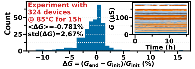
Fig. 6. Experimental results for memory state retention, showing change in device conductance, measured at 0.1 V, after baking for 15 h at 85^\circ\text{C} .
