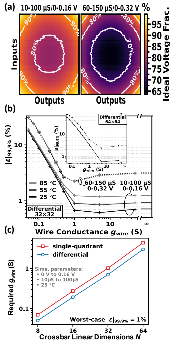
Fig. 4. (a) Heatmap of normalized (by U_{\max} ) average voltages across crosspoint devices in a 64 \times 64 crossbar circuit with g_{\text{wire}} = 0.4 S and double-sided voltage biasing, simulated at room temperature (25 °C), for two different values of U_{\max} and ranges of device conductances. (b) Simulated worst-case error as a function of g_{\text{wire}} for differential 32 \times 32 circuit. Inset shows the results for 64 \times 64 differential crossbar circuit simulated at room temperature. (c) Extrapolated wire conductance g_{\text{wire}} , which is required to ensure the 1% worst-case error.
