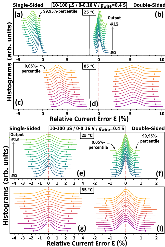
Fig. 3. Simulated results for output current error \varepsilon for (a-d) single-quadrant and (e-i) differential topologies implementing 16 \times 16 VMM. Output #0 (#0 and #15) is the closest to where the input voltages are applied to for single-quadrant (differential) topology. Panels (a, c, e, g) are for single-sided voltage biasing, while (b, d, f, i) are for double-sided ones. Top and bottom panels are for 25 °C and 85 °C, respectively. For all cases, G_{\min} = 10 \mu\text{S} , G_{\max} = 100 \mu\text{S} , and U_{\max} = 0.16 \text{ V} .
