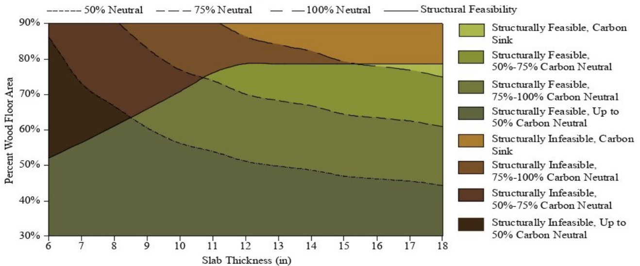
Fig. 5 Carbon-based design for an entire story of the prototypical building
