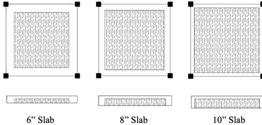
Fig. 3 Plans and sections through one bay of a wood inlay slab for various slab thicknesses
