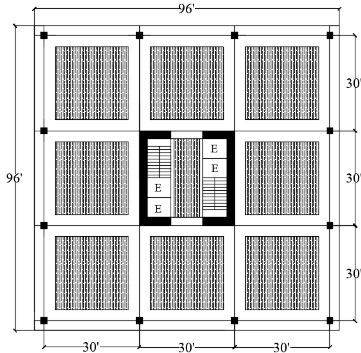
Fig. 2 Typical floor plan of the prototype building - the hatched regions represent the wood inlays in the slab
