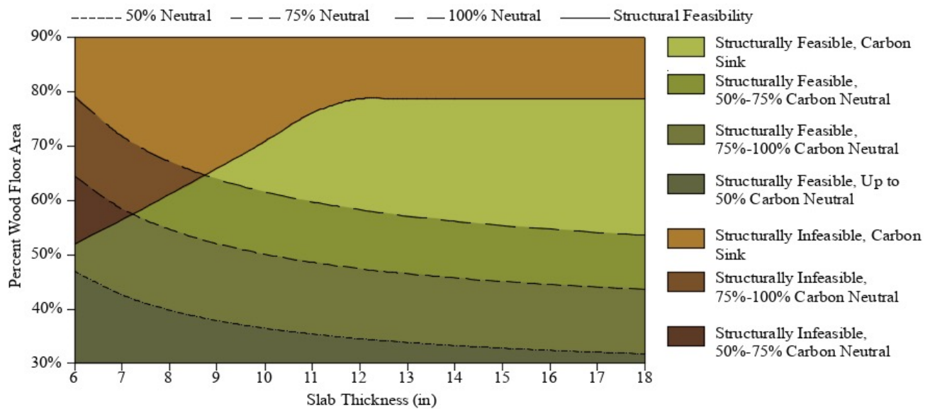
Fig. 4 Carbon-based design chart for the floor slab of the prototype building
