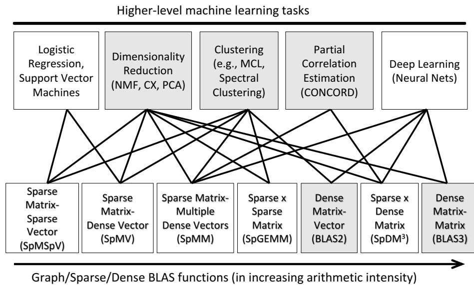
Figure 3. Dependencies of various machine learning methods upon linear algebraic primitives. In the top part, the three boxes in the middle are unsupervised methods whereas the two boxes at the extremes include supervised methods. NMF stands for non-negative matrix factorization, PCA stands for principal component analysis, and MCL stands for the Markov cluster algorithm. CONCORD stands for CONvex CORrelation selection methoD. CX refers to a low-rank matrix factorization in which a subset of the columns (C) is one of the factors.
