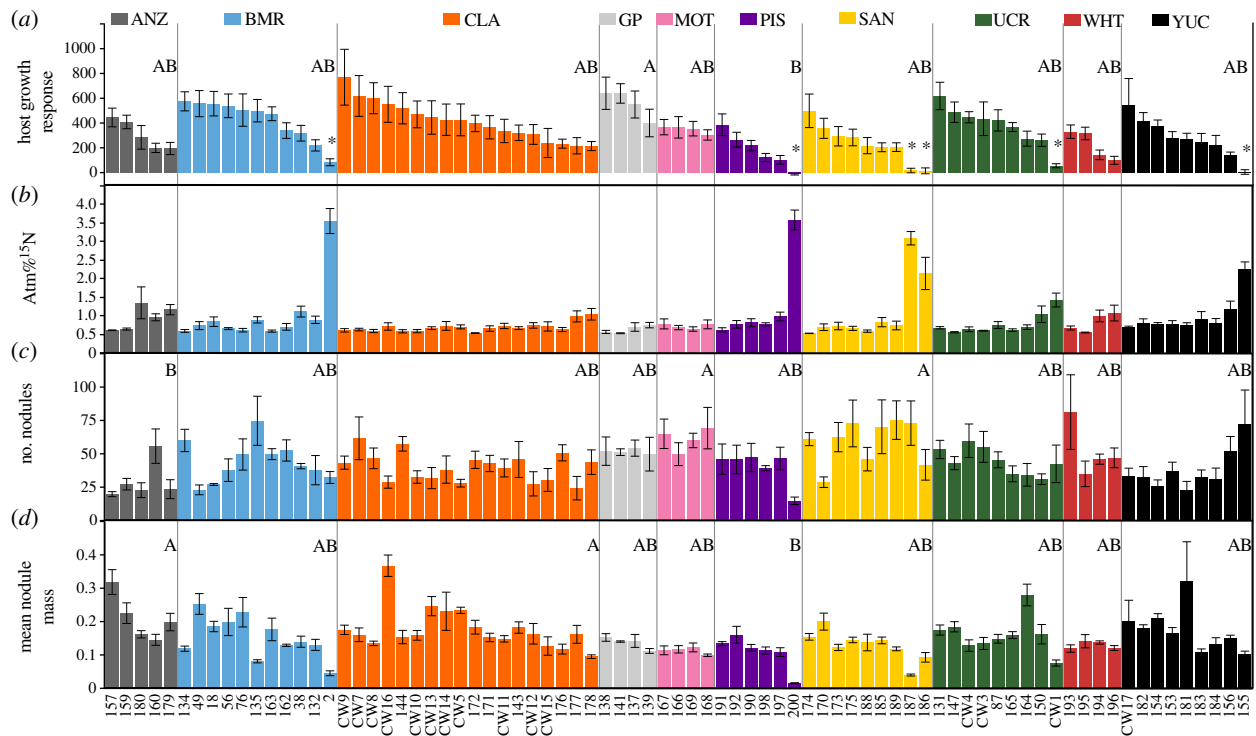
Figure 3. Symbiotic traits of Bradyrhizobium isolates. Host growth response (a), atm% 15 N (b), mean number of nodules formed (c) and mean individual nodule mass (d) are indicated. Colours indicate different field collection sites and asterisks in the host growth response panel identify ineffective isolates. Significant differences among collection sites are indicated with capital letters (electronic supplementary material, table S13). Error bars represent 1 s.e. (Online version in colour.)
