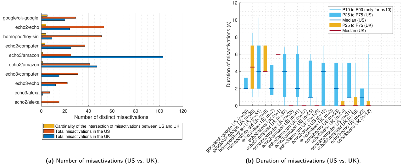
Fig. 10. Misactivation in the US testbed vs. UK testbed: measuring the misactivations differences on US devices vs. UK devices.
