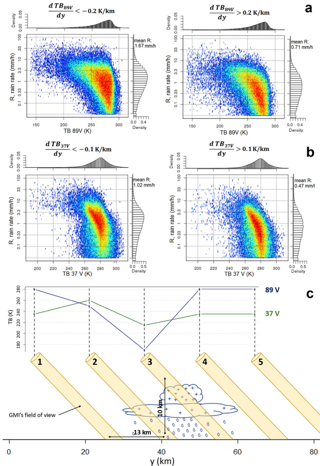
FIG. 9. (a) Joint distributions of DPR surface rain rates and collocated GMI 89V TBs conditioned on the value of the spatial derivative (gradient) of the 89V TB in the azimuthal direction of GMI's observation beam over land: for (left) negative, and (right) positive gradients. (b) Joint distributions of DPR surface rain rates and collocated GMI 37V TBs conditioned on the value of the spatial derivative (gradient) of the 37V TB in the azimuthal direction of GMI's observation beam over land: for (left) negative, and (right) positive gradients. (c) Schematic illustration of
