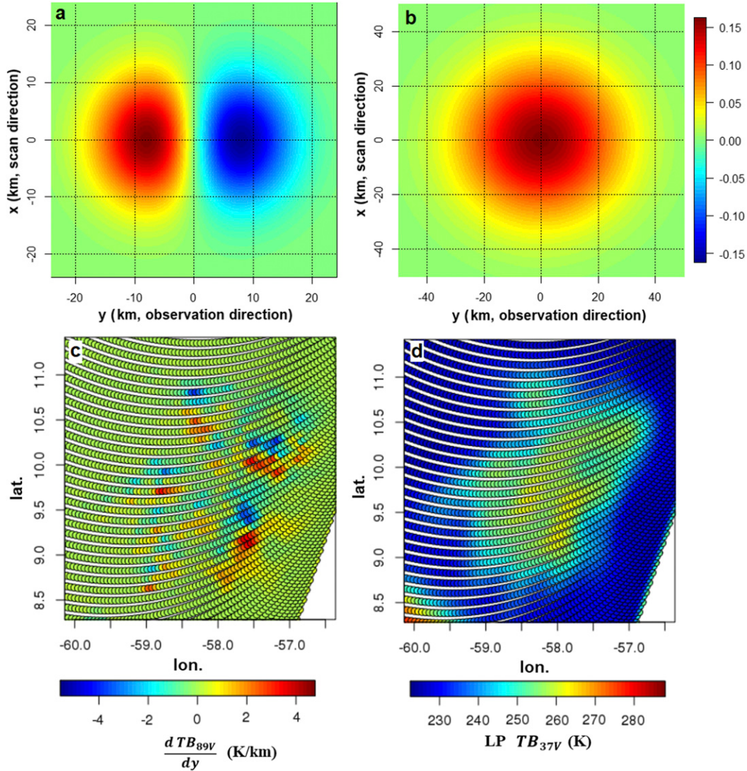
FIG. 8. Convolution kernels used to extract spatial information from the TB fields. (a) First derivative of Gaussian kernel (Szeliski 2010): f(x, y) = -(y/2\pi\sigma^4)e^{-[(x^2+y^2)/2\sigma^2]} with \sigma = 8 km; this kernel is convolved with the 37 and 89V TB fields. (b) Gaussian kernel (Szeliski 2010): f(x, y) = (1/2\pi\sigma^2)e^{-[(x^2+y^2)/2\sigma^2]} with \sigma = 20 km; this kernel is convolved with the 37 V TB field. (c) Result of the convolution of the 89V TB field shown in Fig. 6 (bottom) with the First derivative of Gaussian kernel. (d) Result of the convolution of the 37V TB field shown in Fig. 6 (top) with the Gaussian kernel. The Gaussian smoothing kernel partially erases the ice-scattering signal at 37 GHz. In (a) and (b), the x direction is tangent to the imager's scan (orthogonal to the observation direction) and the y direction is along the azimuthal direction of the imager's observation beam (orthogonal to the scan).
