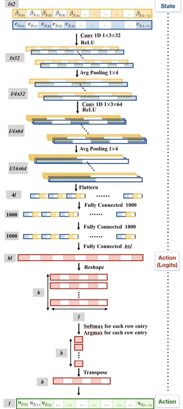
Fig. 8. Structure of the actor network \mu(\cdot|\theta_u) .
