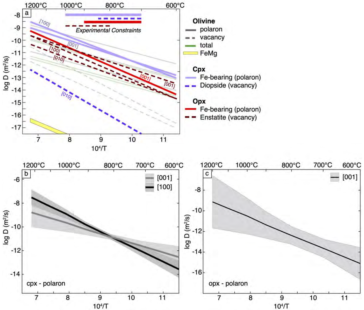
Figure 2: (a) Arrhenius diagram showing H^+ diffusion rates in clinopyroxene (Jaipur diopside for the proton-polaron mechanism, Woods et al. 2000; Ferriss et al. 2016 and synthetic diopside for the proton vacancy mechanism, Sundvall et al. 2009) and orthopyroxene (Kilbourne Hole enstatite for the proton-polaron mechanism, Stalder and Skogby 2003 and synthetic enstatite for the proton-vacancy mechanism, Stalder and Behrens 2006) overlaid on the olivine mechanisms (Mackwell and Kohlstedt 1990; Demouchy and Mackwell 2006; Ferriss et al. 2018). Olivine D_{FeMg} is shown for comparison (Dohmen and Chakraborty 2007a, 2007b). Isotropic data (or experimental datasets where only one crystallographic axis has an Arrhenius relationship constrained) have one line, while anisotropic diffusivities have multiple lines for different crystallographic axes. Experimental constraints between 700-1000°C (shown at the top of the figure) were used to extrapolate using the log-linear Arrhenius relationships. (b) Clinopyroxene proton-polaron and (c) orthopyroxene proton-polaron Arrhenius relationships are shown with 95% confidence interval error envelopes (shaded fields) calculated from experimental data.
