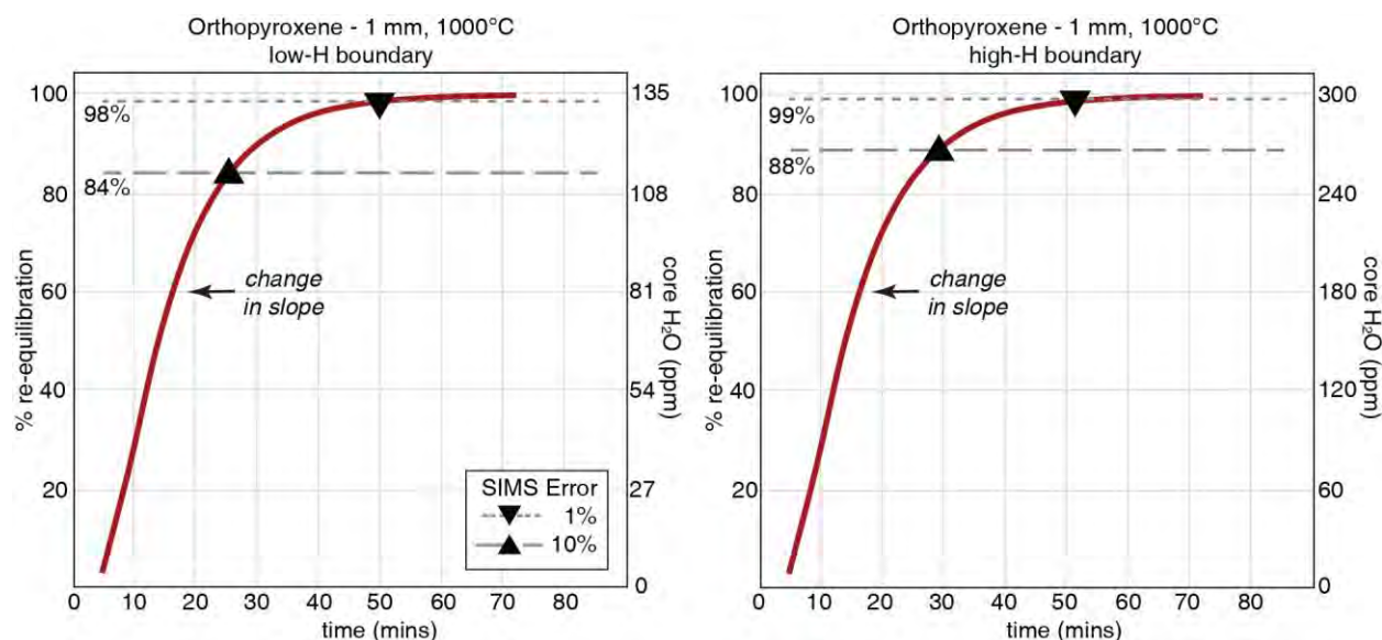
Figure 7: Orthopyroxene re-equilibration with diffusion time for the low-H (left) and high-H (right) boundary conditions using the proton-polaron diffusion coefficient. Black downward pointing triangles (1% analytical error) and upward-pointing triangles (10% analytical error) indicate the effective %re-equilibration point for each model, where any zonation beyond that value would be difficult to resolve outside of analytical error. For the low-H boundary, 1% analytical error intersects the modeled re-equilibration line after 50 minutes of diffusion, which is a 30% shorter duration compared to the 100% re-equilibration time of 72 minutes (Table 2). The 10% error intersects the re-equilibration line after ~25 minutes, representing a duration that is about 65% shorter compared to the 100% time. For the high-H boundary, 1% error intersects the modeled re-equilibration line after ~52 minutes, and 10% error intersects at ~28 minutes (Supplementary Table S4).
