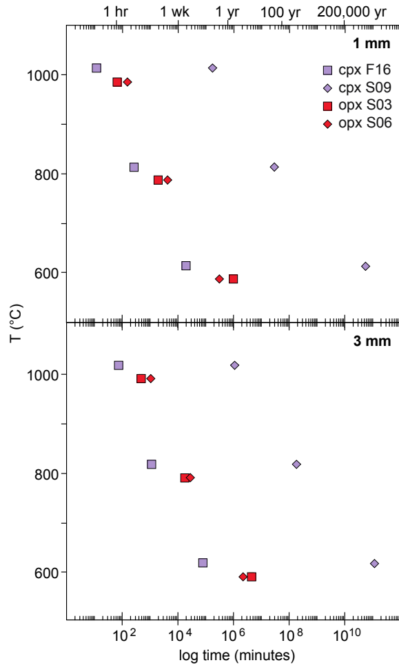
Figure 6: Model results for proton-polaron diffusion mechanisms (squares) compared to possible proton-vacancy diffusion mechanisms (diamonds) for 1 and 3 mm pyroxene models. Proton-polaron models (square symbols) are as shown in Figure 5. Models representing the proton-vacancy mechanism utilize Sundvall et al. (2009; purple diamonds) for cpx and Stalder and Behrens (2006; red symbols) for opx. Legend abbreviations are: F16 – Ferriss et al. 2016; S09 – Sundvall et al. 2009; S03 – Stalder and Skogby 2003; S06 – Stalder and Behrens 2006.
