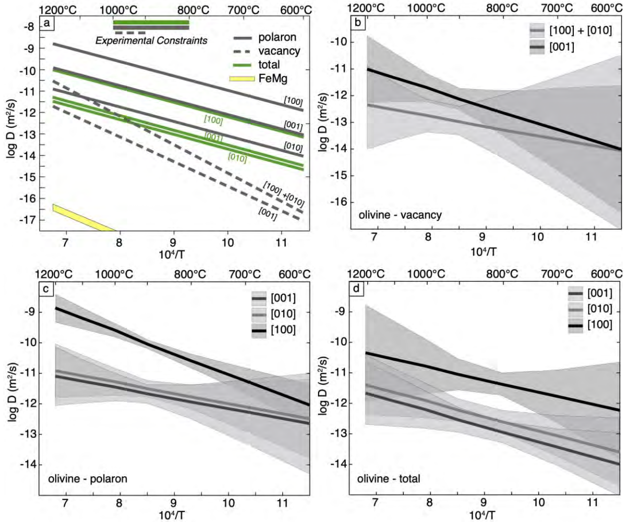
Figure 1: Arrhenius diagram showing H + diffusion rates in olivine for the proton polaron mechanism (solid grey lines - Mackwell and Kohlstedt 1990), proton vacancy mechanism (dashed grey lines - Demouchy and Mackwell 2006), and total H + diffusion (green lines - Ferriss et al. 2018). Olivine D_{\text{FeMg}} (yellow region) is shown for comparison (Dohmen and Chakraborty 2007a, 2007b). Anisotropic diffusivities are labeled for each principal crystallographic axes. Experimental constraints between 800-1000°C (shown at the top of the figure) were used to extrapolate using the log-linear Arrhenius relationships. Uncertainties associated with this extrapolation are represented by 95% confidence interval error envelopes (shaded fields) calculated from experimental data for the (b) proton vacancy mechanism, (c) proton polaron mechanism, and (d) "total" H diffusion.
