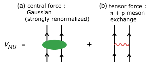
FIG. 23. Diagrams for the V_{MU} interaction. From Otsuka, Suzuki, Honma et al. , 2010.
