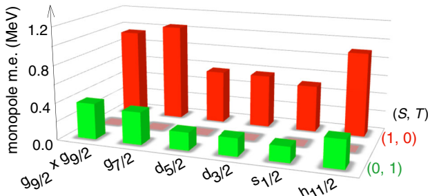
FIG. 12. Monopole matrix elements of delta interactions for (S, T) channels. See the caption of Fig. 11.
