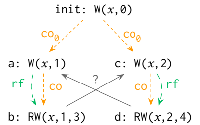
Fig. 4. Concurrent Read-writes
