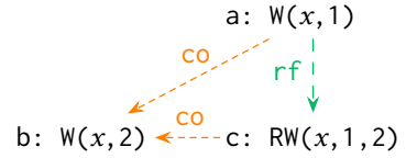
Fig. 13. Read-write Exclusivity
