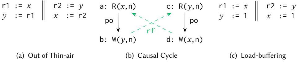
Fig. 3. Causal Cycles
