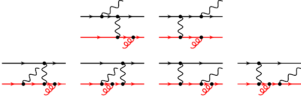
Fig. 4. LO diagrams for the subprocess \ell q g \rightarrow \ell q \gamma . The hard photon can either be radiated of the lepton (black fermion line) or the quark (red fermion line).
