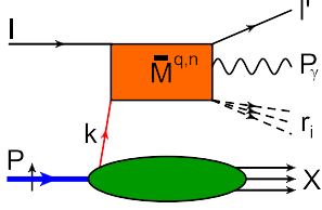
Fig. 1. Factorized amplitude with one quark leg connecting the nucleon (green blob) and the hard scattering amplitude \mathcal{M}^{q,n} .
