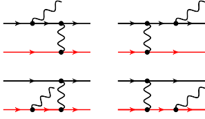
Fig. 2. LO diagrams for the subprocess \ell q \rightarrow \ell q \gamma . The photon can either be radiated off the lepton (black fermion line) or the quark (red fermion line).
