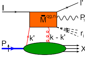
Fig. 3. Factorized amplitude with a quark and a gluon leg connecting the nucleon (green blob) and the hard scattering amplitude \mathcal{M}^{qg,n} .
