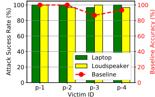
Figure 10: Results of attacking live human speech.
