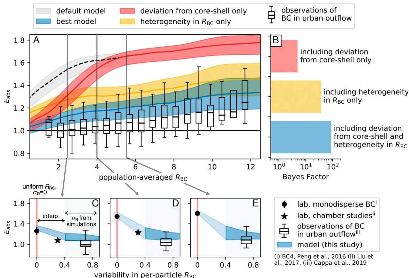
Fig. 2. The previously reported gap between modeled and observed E_{\text{abs,bulk}} (illustrated here by comparison of the dashed black line with the box plot in A) is largely reconciled by the improved model (blue line and shading in A), which accounts for both heterogeneity in R_{\text{BC}} and deviations from the core-shell approximation. This improved model is compared with the default model (black line), which assumes a core-shell configuration and neglects particle-to-particle diversity entirely. Evaluation of two additional cases in which only deviation from the core-shell approximation is considered (red shading in A and B) and in which only heterogeneity in composition is considered (yellow shading in A and B) shows that neglecting variability in per-particle R_{\text{BC}} is the primary cause of differences in modeled and observed E_{\text{abs,bulk}} . Differences in E_{\text{abs,bulk}} between different particle populations having the same R_{\text{BC,bulk}} —both calculated and observed—are explained by differences in the variability in per-particle R_{\text{BC}} (C–E) between populations. Populations having large variability in per-particle R_{\text{BC}} , as expected among ambient BC, are predicted to have weaker levels of E_{\text{abs,bulk}} than populations having lower variability in per-particle R_{\text{BC}} . Variability in R_{\text{BC}} was estimated by fitting the ambient distributions in R_{\text{BC}} reported in ref. 7. In all cases, the best estimate (lines) and 1 - \sigma bounds (shading) were determined from a Bayesian regression of the particle-resolved model data, and the observational strength of one model over another is quantified using the Bayes factor ( Methods ). The measurements and model calculations shown here were performed at a wavelength of 532 nm.
