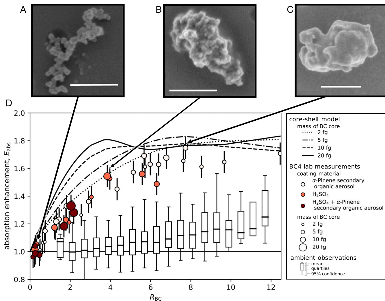
Fig. 1. The complex, noncore-shell morphology of BC-containing particles (A–C) leads to lower enhancements in light absorption (denoted E_{\text{abs}} ; circles in D) than predicted under the core-shell approximation (black lines in D) for a given R_{\text{BC}} , consistent with findings reported in refs. 6, 7, and 34. However, both the core-shell model and the measurements from the BC4 experiment predict larger E_{\text{abs}} for the same R_{\text{BC}} than has been observed in ambient populations (shown by boxes in D) for BC sampled in urban outflow near Fontana, CA (10). The R_{\text{BC}} values for the ambient measurements are ensemble averages. The BC4 measurements provide E_{\text{abs}} for mass-selected BC cores, where the mass of the BC core, amount of coating, and composition of the coating varied between experiments. Particles were also imaged periodically to capture the internal morphology of the laboratory-generated particles (A–C). The model calculations and measurements shown here were performed at a wavelength of 532 nm. (Scale bars: A–C, 300 nm.)
