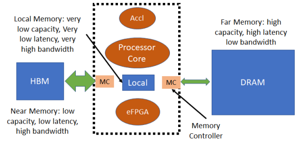
Figure 9: Target architecture.
