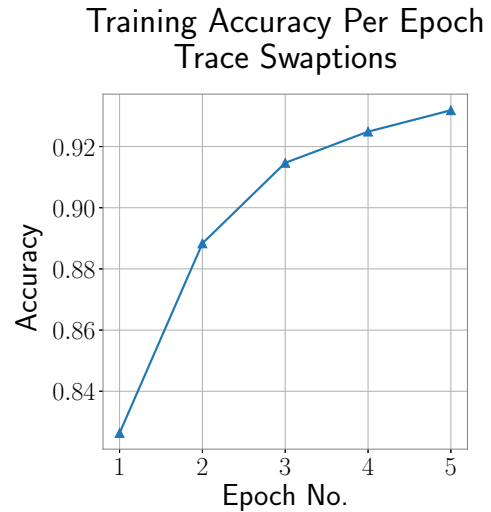
Figure 4: Training accuracy per training epoch for the Swaptions app. Five epochs appear to be enough for the training accuracy to start stabilizing.
