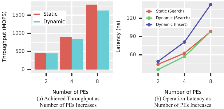
Fig. 9. Evaluation of static and dynamic hash table on Intel Stratix 10 FPGA. Parameters: key/value length: 32-bit. 4 slots/entry (dynamic hash table).
