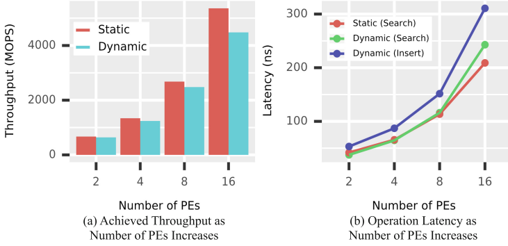
Fig. 7. Evaluation of static and dynamic hash tables on Xilinx U250 FPGA. Parameters: key/value length: 32-bit. 4 slots/entry (dynamic hash table).
