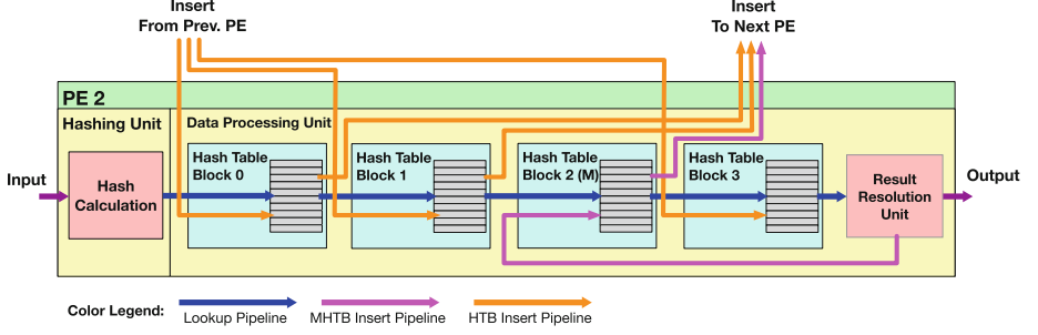
Fig. 4. Architecture of PE 2 in a 4 PEs design. Master Hash Table Block (MHTB) ID is 2 in this case.
