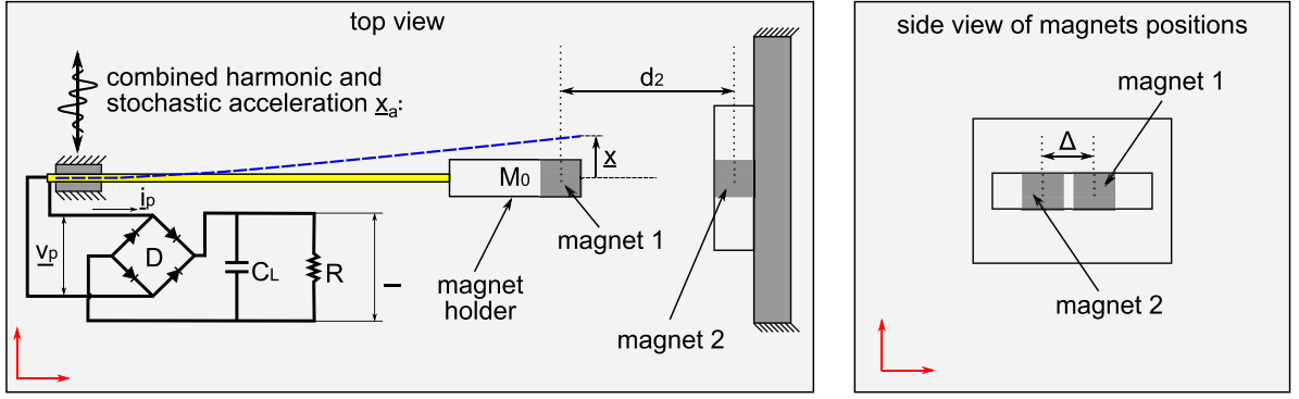
Fig. 1. Schematic of nonlinear energy harvesting system.
