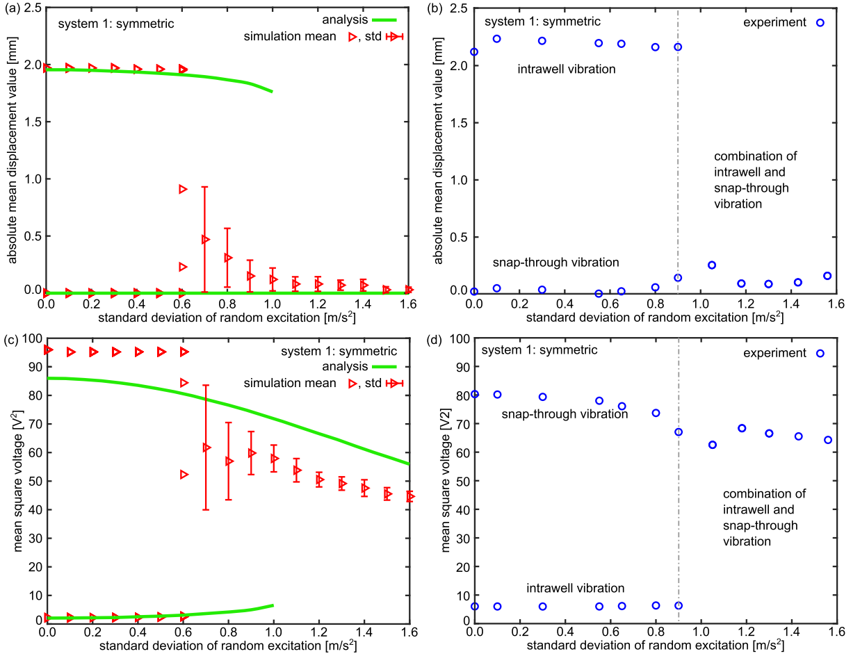
Fig. 4. Responses for system 1 with harmonic base acceleration amplitude 3.3 \text{ m/s}^2 at frequency 9 \text{ Hz} . Absolute mean value of displacement amplitude from (a) analysis and simulation and (b) experiment. Mean-square of total rectified voltage from (c) analysis and simulation and (d) experiment.
