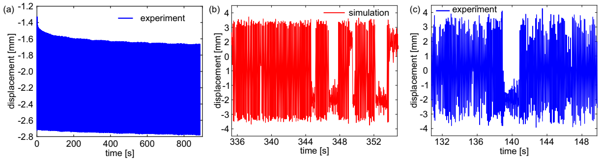
Fig. 5. Transient displacements from (a) experiment under pure harmonic excitation, (b) simulation and (c) experiment at harmonic excitation amplitude 3.3 m/s 2 and noise standard deviation 1.6 m/s 2 .
