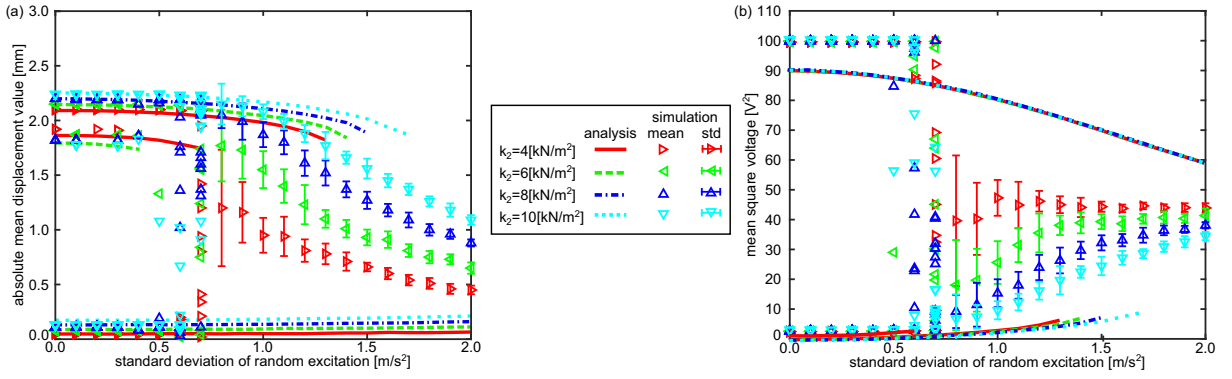
Fig. 11. Analytical and numerical responses for four asymmetrical energy harvesting systems with harmonic amplitude 3.3 \text{ m/s}^2 and frequency 9 \text{ Hz} . (a) Absolute mean value of displacement amplitude. (b) Mean square voltage.
