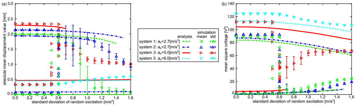
Fig. 12. Analytical and numerical responses for system 1 and 2 at frequency 9 \text{ Hz} and system 3 at 10 \text{ Hz} . (a) Absolute mean value of displacement amplitude. (b) Mean square voltage.
