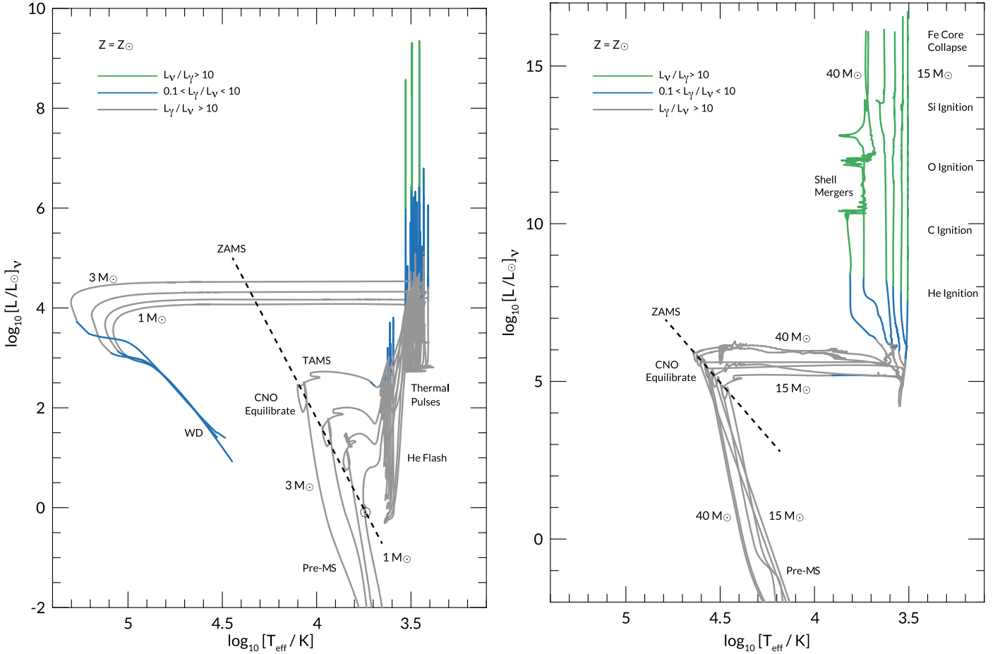
Figure 4. Ratio of the photon luminosity to the neutrino luminosity in a neutrino H-R diagram. Low-mass stars are on the left, high-mass stars on the right. Gray curves indicate where photons dominate, green curves where neutrinos dominate, and blue curves where the photon and neutrino luminosities are within a factor of 10. The neutrino luminosity is normalized by the current solar value L_{\nu,\odot} = 0.02398 \cdot L_{\gamma,\odot} = 9.1795 \times 10^{31} \text{ erg s}^{-1} (see Section 2.2).
