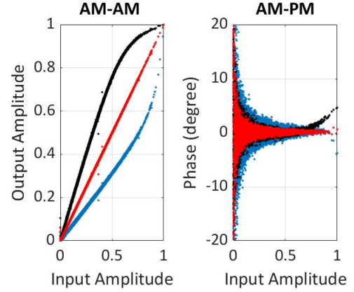
Fig. 4: Dynamic AM-AM and AM-PM curves of ZFL-2500 amplifier without (black) and with (blue) DPD (red).
