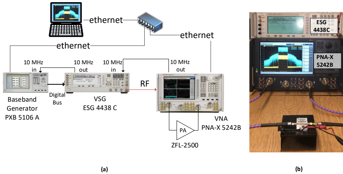
Fig. 1: (a) Schematic and (b) picture of the testbed used for the measurements.
