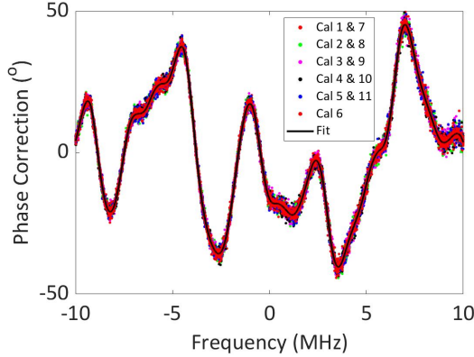
Fig. 3: Phase calibration \phi_{\text{CAL}} corrections obtained for 11 different measurements.
