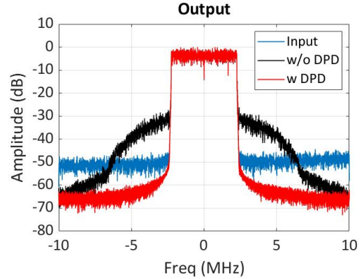
Fig. 5: Spectra of ZFL-2500 amplifier before and after DPD.
