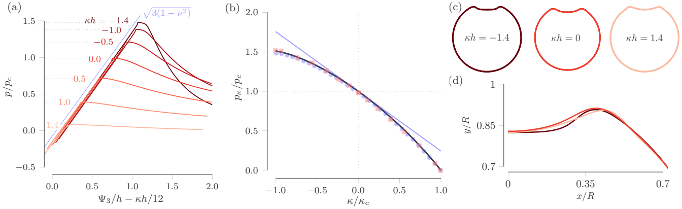
FIG. 3. (a) Plots of the pressure normalized by p_c as a function of the normal displacement of the shell at its apex. The critical pressure p_c is given by Eq. (86) and the normal displacement along the x axis is given according to Eq. (53). As normalized, the slope of the fundamental state is given by \sqrt{3(1-\nu^2)} . We note that the slope of the post buckling curve becomes very steep for large, negative values of \kappa h , and is nearly flat, but still decreasing, for large, positive values of \kappa h . (b) The theoretical curve from Eq. (85), along with its linearized form given by Eq. (88). The x axis is normalized by the critical buckling curvature, given by Eq. (87). Numerical results from the 1D axisymmetric model (●) and the 2D model (■) coincide directly with the analytical prediction. (c) Postbuckling shapes from the 1D model at \Psi_3/h = 20 for three different values of \kappa h . (d) Profiles of the the postbuckling shapes that have been magnified near the shell's apex.
