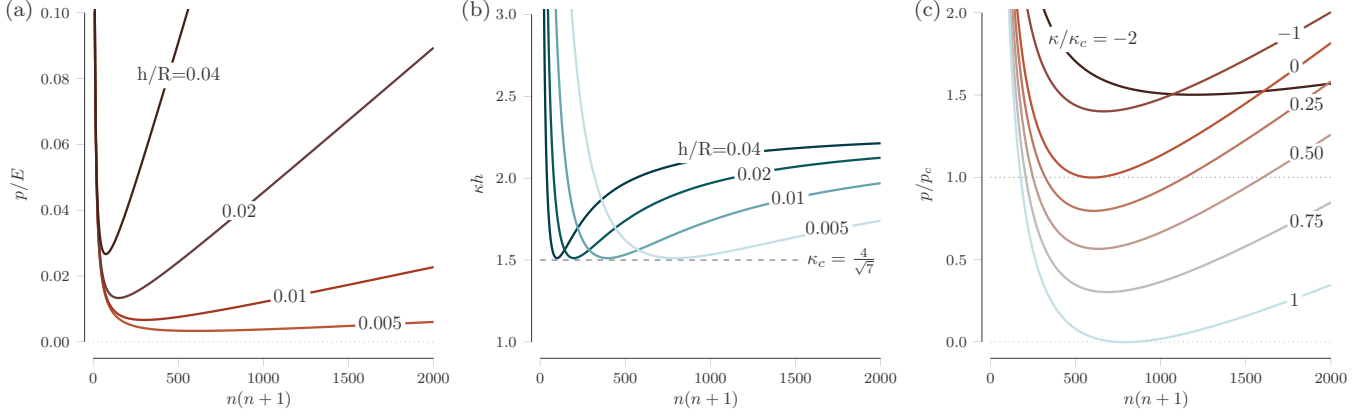
FIG. 2. (a) A plot of externally applied pressure p normalized by the Young's modulus E as a function of eigenmodes written as n(n+1) for several values of h/R . This plot is the classical result in the absence of natural curvature \kappa . (b) A plot of natural curvature \kappa normalized by h as a function of eigenmodes written as n(n+1) for several values of h/R . This plot is in the absence of external pressure, and recreates the results from Ref. [44]. (c) A plot illustrating the coupling of pressure and curvature. Here the pressure is normalized by the classical buckling pressure given by Eq. (86) and is plotted against eigenmodes written as n(n+1) for several values of natural curvature normalized by the critical buckling curvature \kappa_c = 4/\sqrt{7} . These curves are plotted from Eq. (83).
