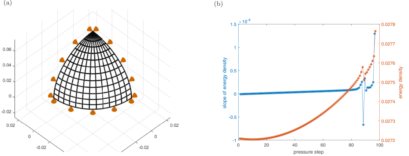
FIG. 4. (a) The one-eighth symmetric geometry model with brown arrows denoting its symmetry planes. (b) The critical points during multiple pressure steps due to the buckling.
