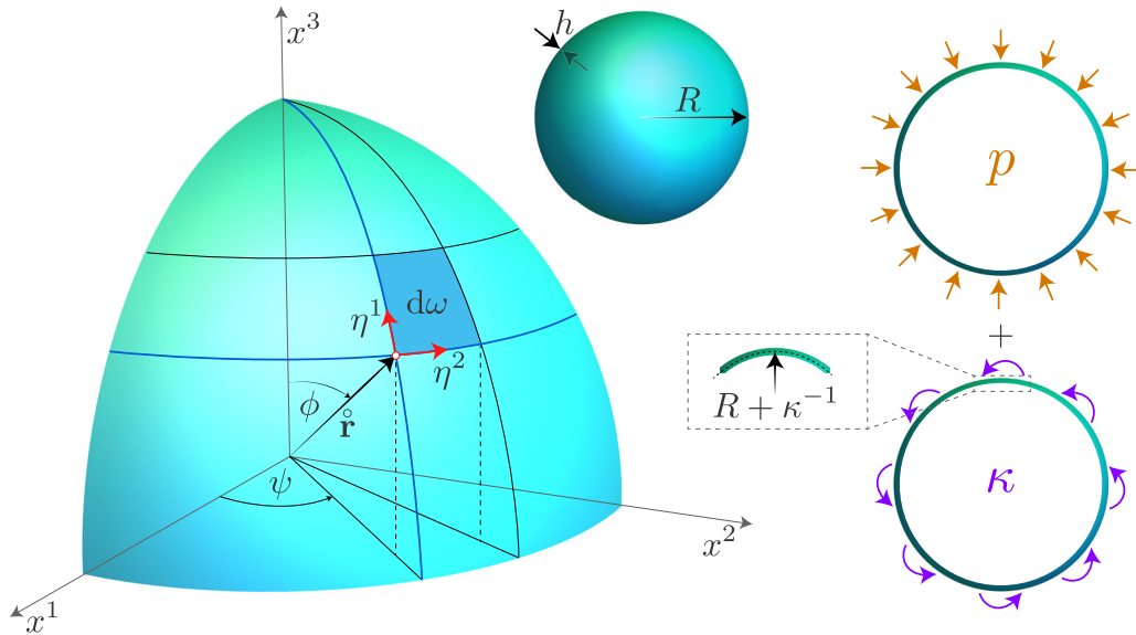
FIG. 1. A schematic of a spherical shell (inset) along with a shell segment denoting the curvilinear coordinates \eta^\alpha at a point a distance \hat{r} from some origin in space.
