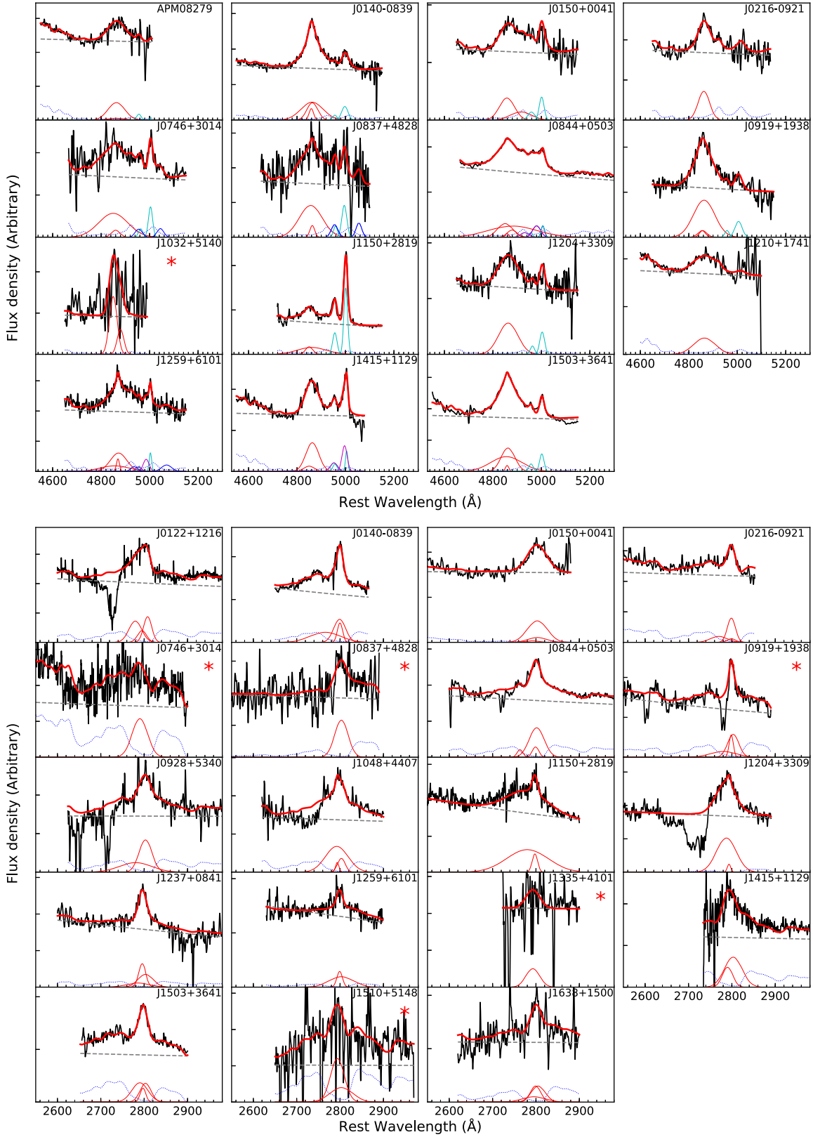
Figure 4. Spectral fits around the H\beta + [O III] (upper panel) and Mg II (lower panel) emission lines in our sample. The model of the H\beta emission line includes the power-law continuum (gray dashed), optical Fe II template (dotted blue), multiple Gaussians for the broad H\beta line (thin red), [O III] \lambda 4960/5008 doublet (cyan and magenta lines, in which magenta lines represent broad FWHM components of the [O III] \lambda 4960/5008 doublet lines), and an additional two broad Gaussians for Fe II bumps at 4940 and 5040 Å (solid blue), if they exist. The model of the Mg II emission line includes the power-law continuum (gray dashed), UV Fe II template (dotted blue), and multiple Gaussians for the broad Mg II line (thin red). The red asterisks refer to objects with low-S/N spectra and/or absorption attached on the line.
